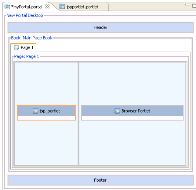
Figure 3-14 Portal in Editor View with Portlets Added
