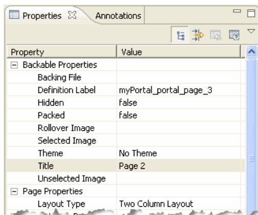
Figure 3-4 Changing a Page Title in the Workbench Properties View
