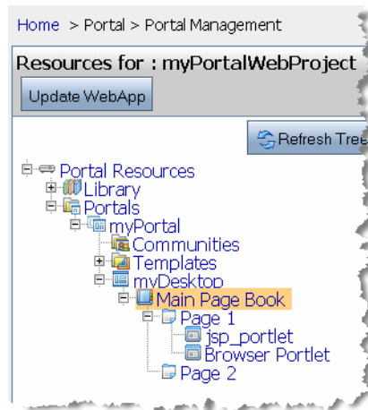
Figure 4-7 Expanded Portal Resources Tree Showing Desktop Pages
