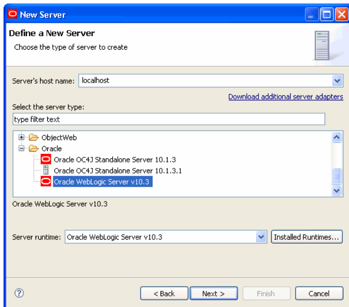
Figure 2-2 New Server – Define a New Server Dialog
