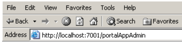
Figure 3 Localhost URL
