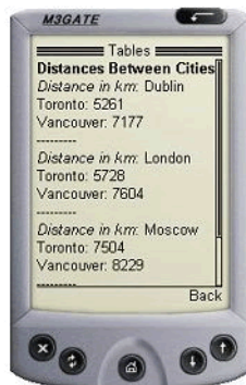
Figure 37 Distances table with bodylocation=1 5 6 and major=row
