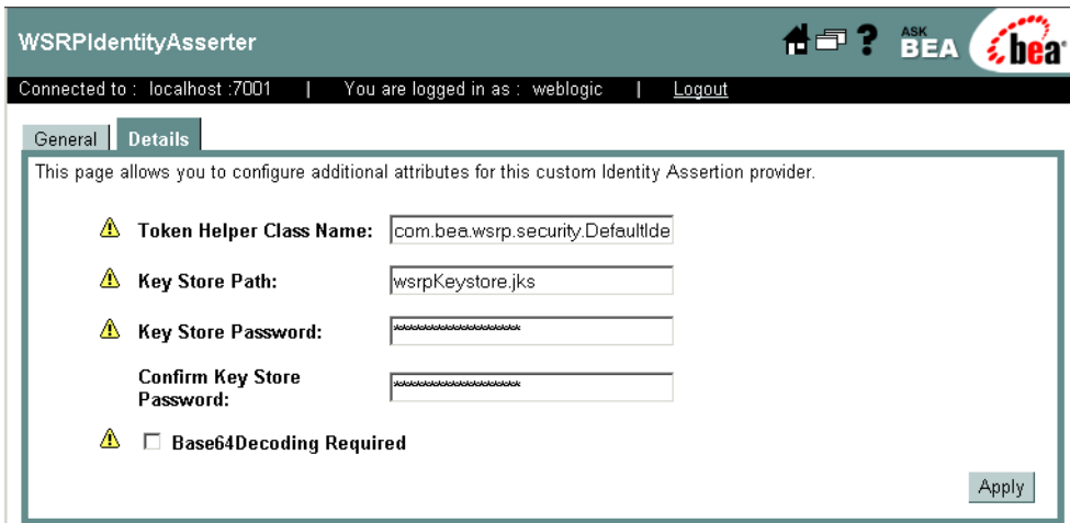
Figure 9-26 WSRP Identity Asserter Detail
