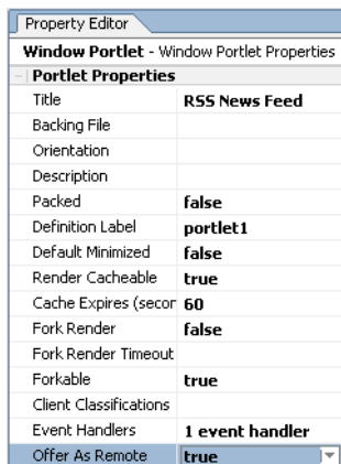
Figure 4-4 Proxy Portlet Property Editor—Offer as Remote Property Selected
