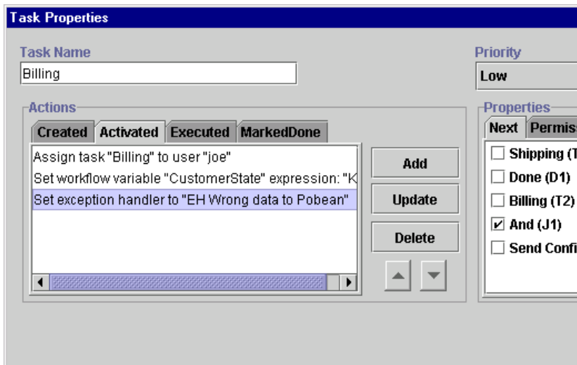
Figure 4-7 Billing Task Properties Dialog Box: Activated Tab
