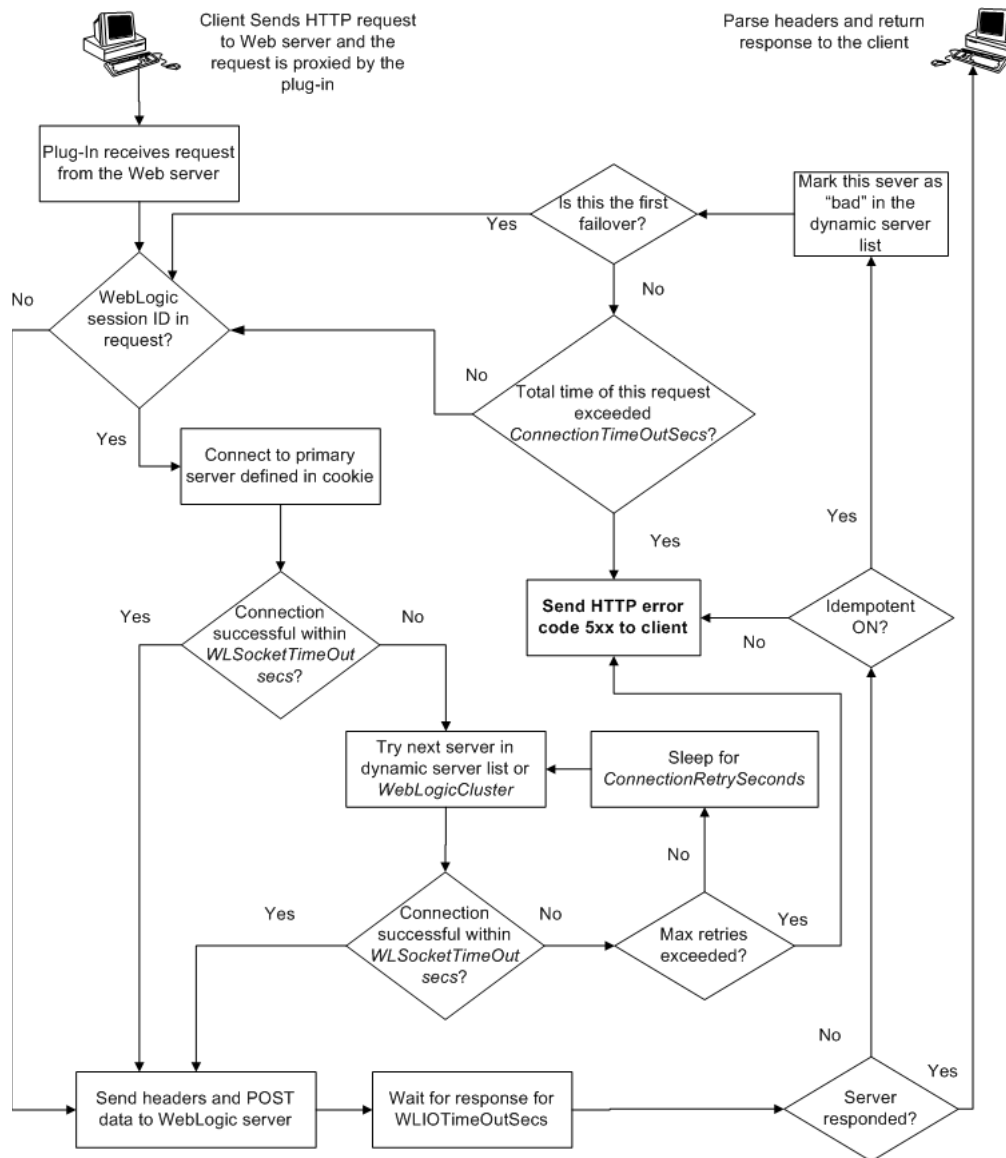
Figure 3-1 Connection Failover
