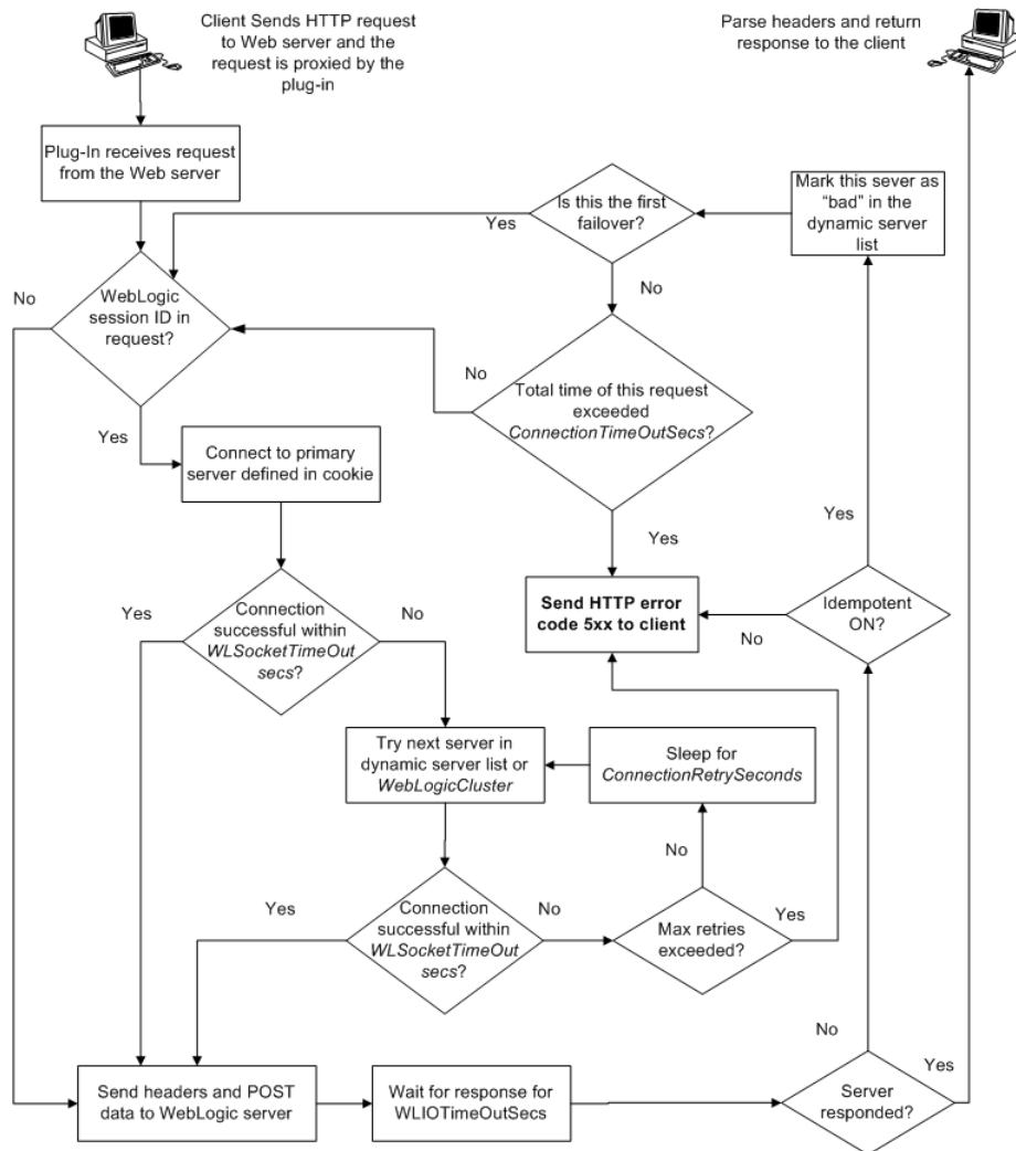
Figure 4-1 Connection Failover
