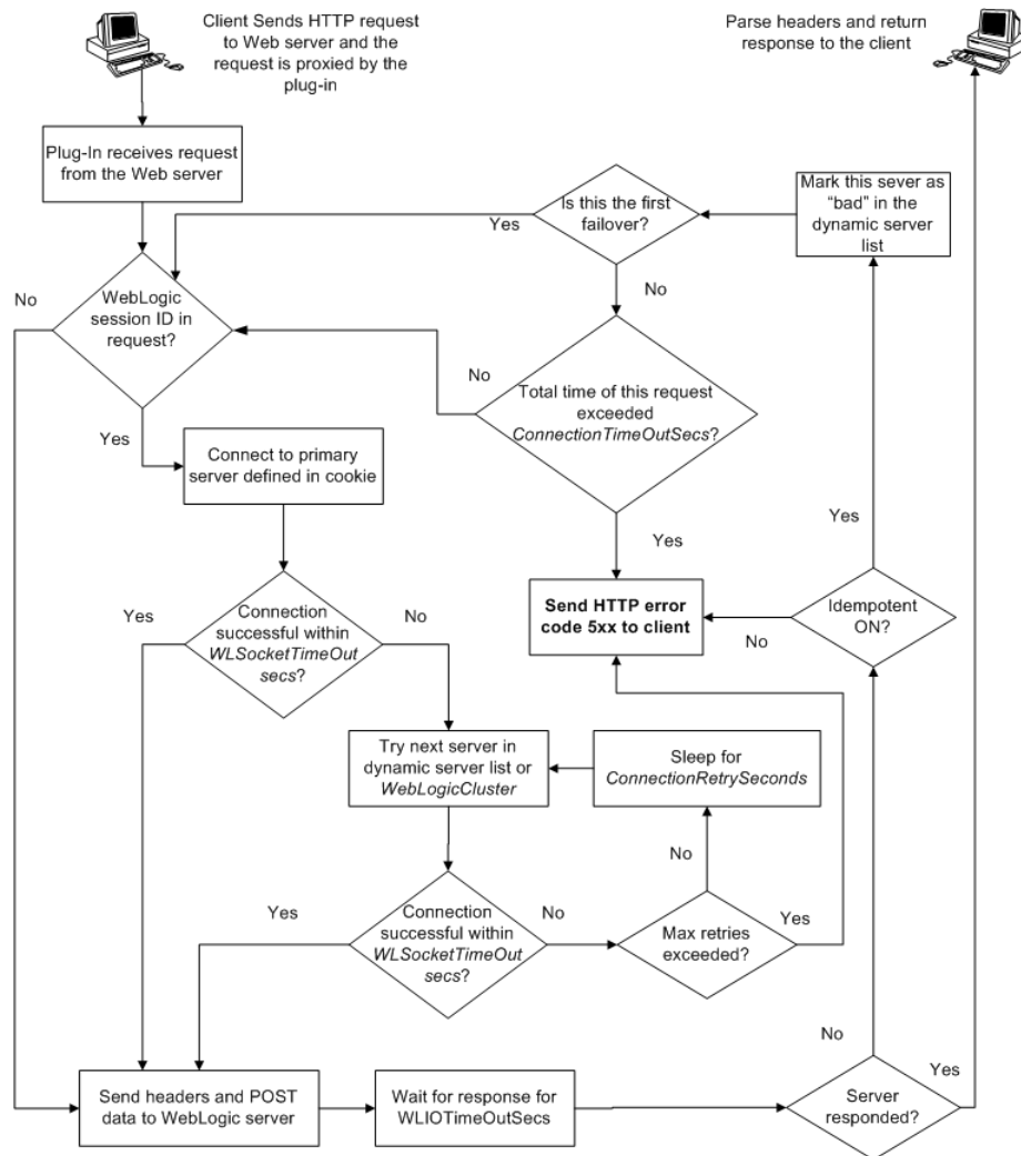
Figure 5-1 Connection Failover
