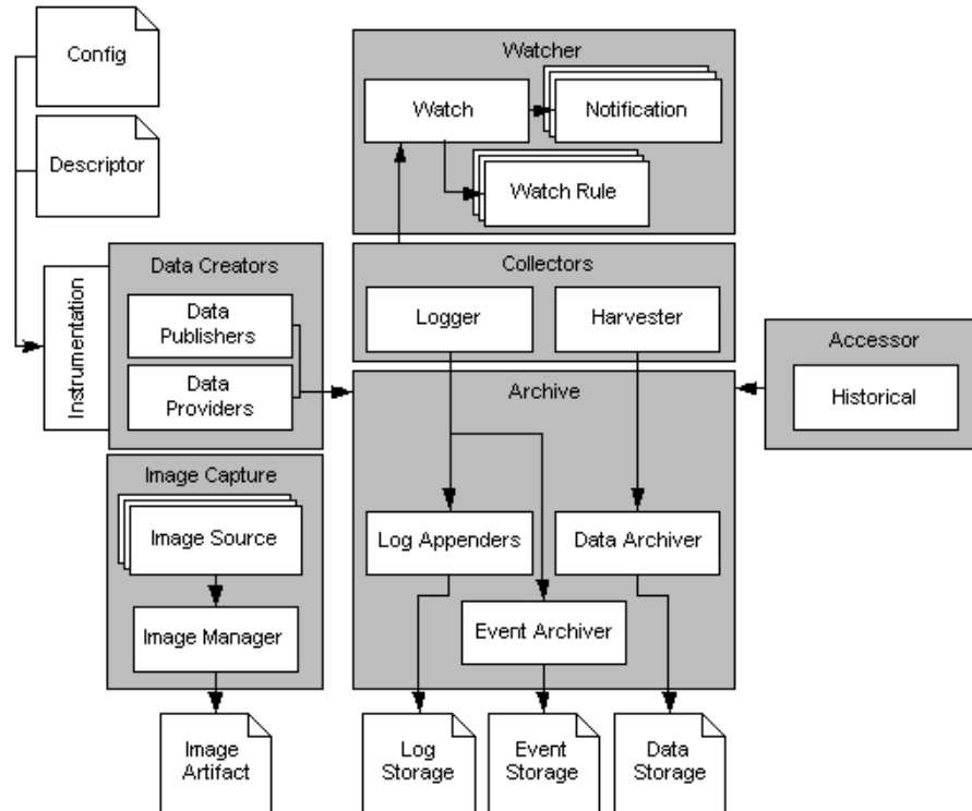
Figure 2-7 Overall View of the WebLogic Diagnostic Framework
