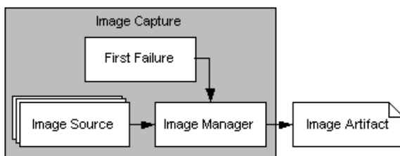
Figure 2-6 Diagnostic Image Capture
