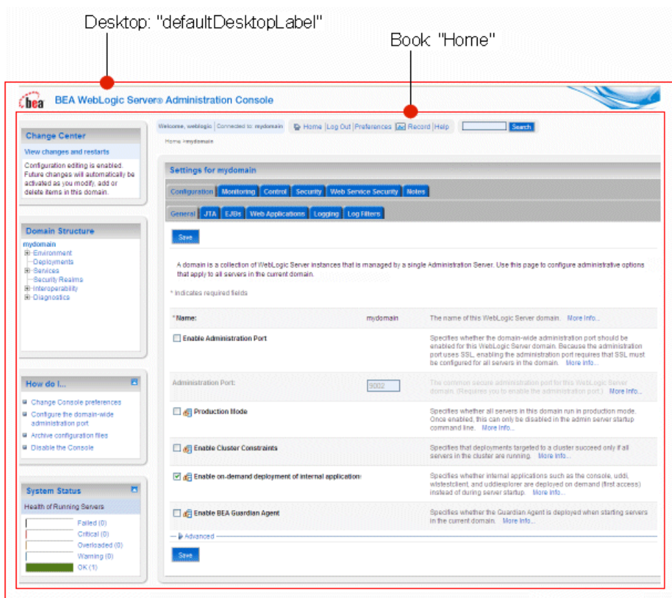
Figure 2-2 The Desktop
