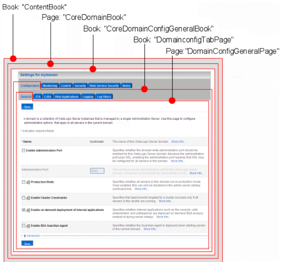
Figure 2-4 The ContentBook
