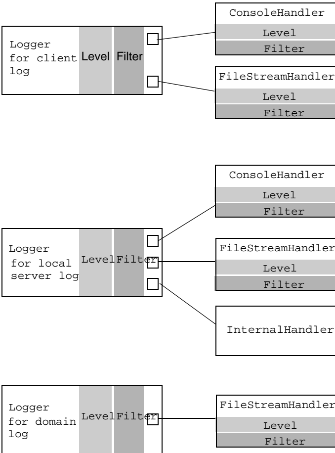
Figure 4-1 WebLogic Logging Services Contexts
