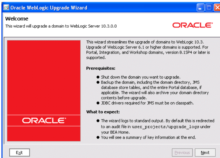
Figure 5-1 WebLogic Upgrade Wizard
