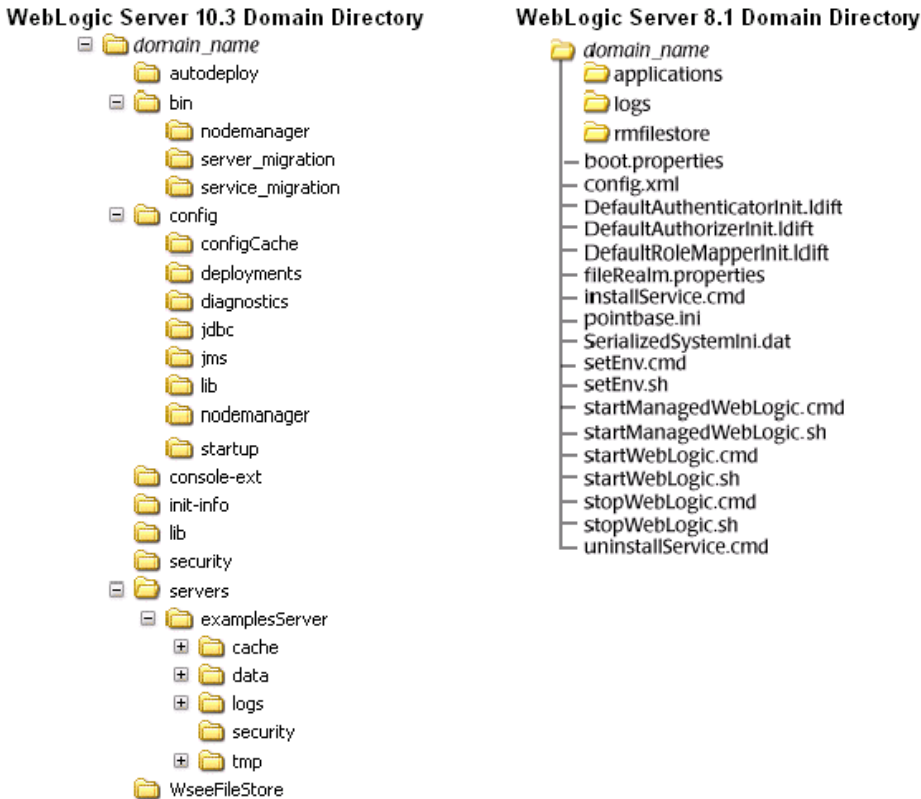
Figure C-1 WebLogic Server 10.3 and WebLogic Server 8.1 Directory Structures
