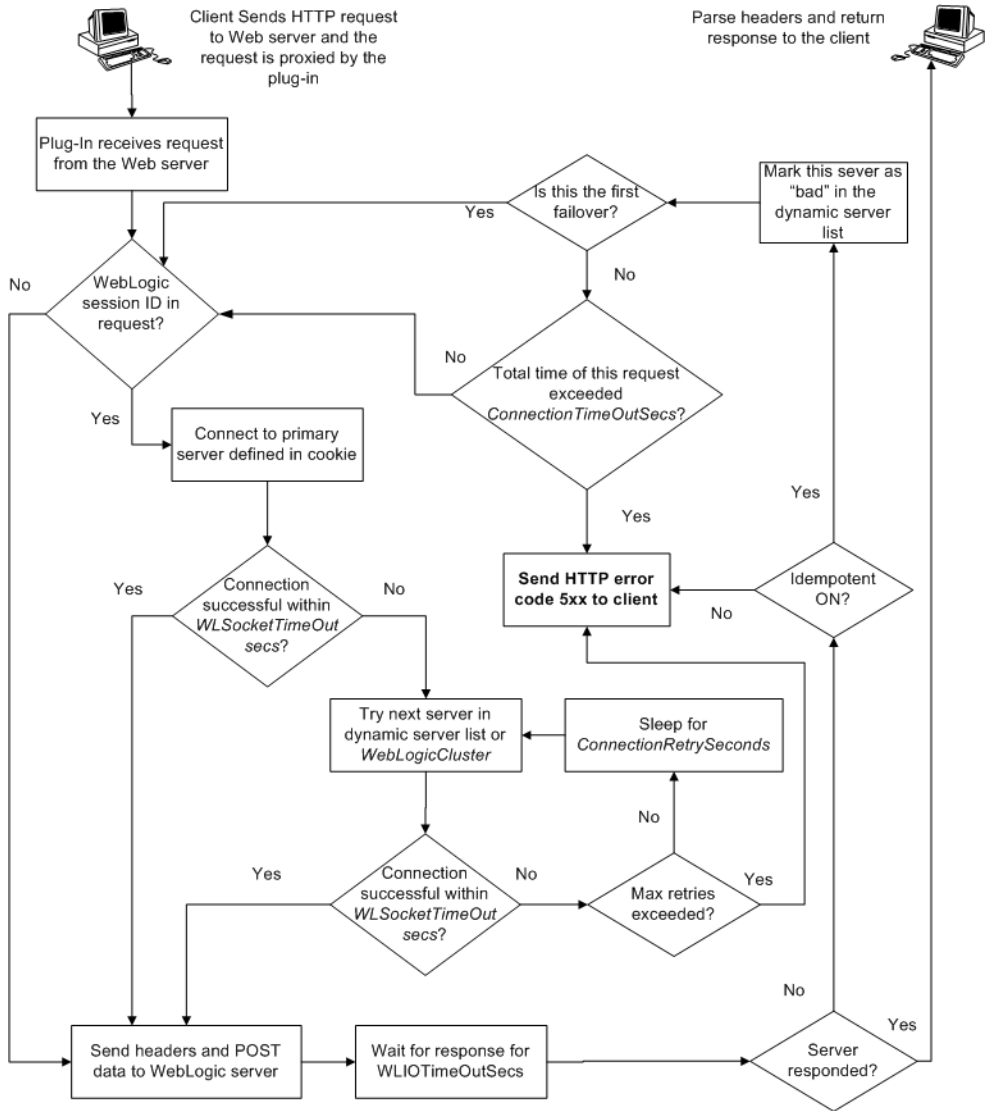
Figure 4-1 Connection Failover
