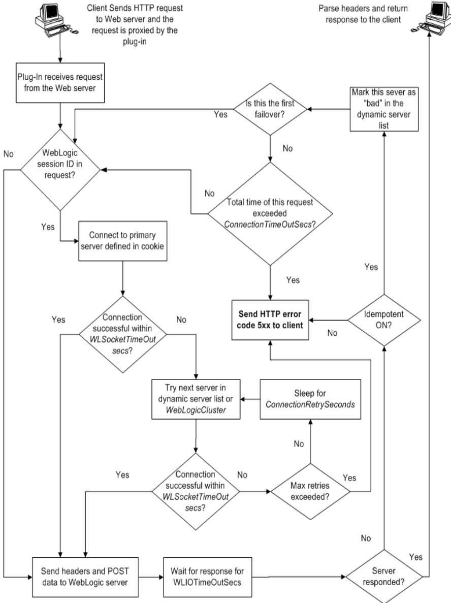
Figure 3-1 Connection Failover
