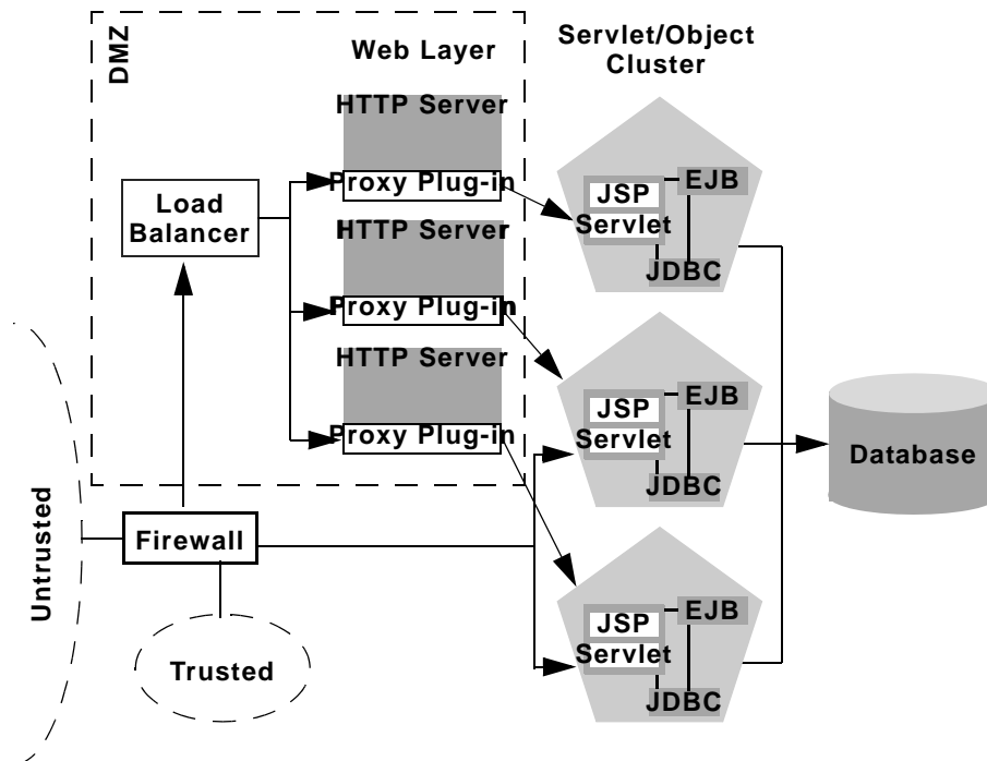
Figure 7-9 Application Components Have Restricted Access Through Firewall
