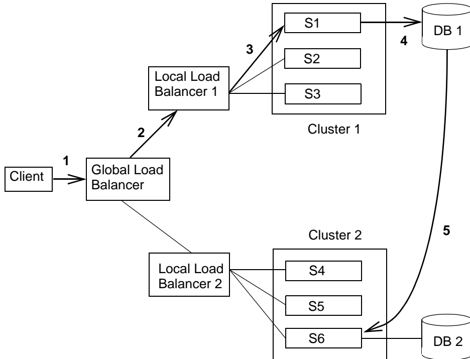
Figure 6-7 WAN Replication
