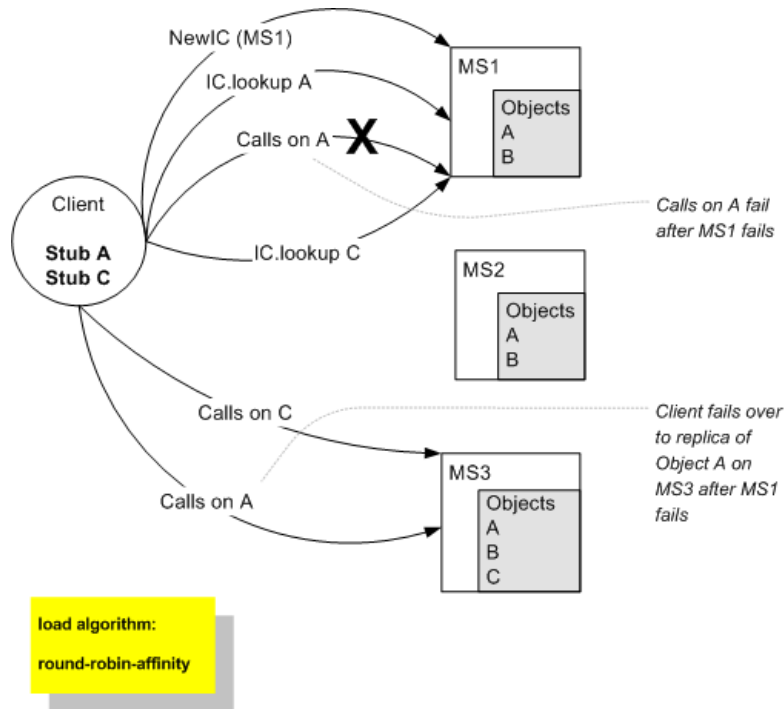
Figure 5-3 Server Affinity and Server-to-Server Connections
