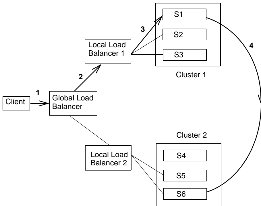
Figure 6-6 MAN Replication
