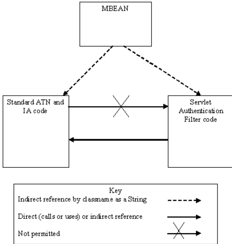
Figure 12-1 Authentication Providers Do Not Call Servlet Authentication Filters
