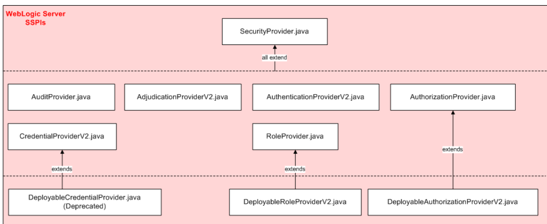
Figure 2-2 “Provider” SSPIs
