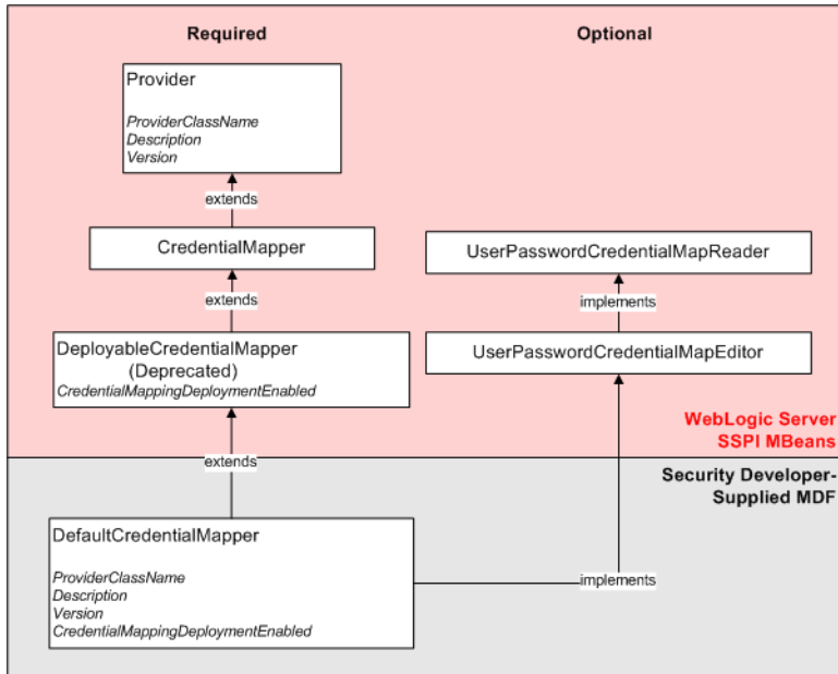
Figure 2-5 SSPI MBean Hierarchy for Credential Mapping Providers
