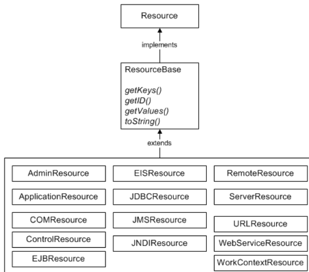
Figure 2-10 Architecture of WebLogic Resources
