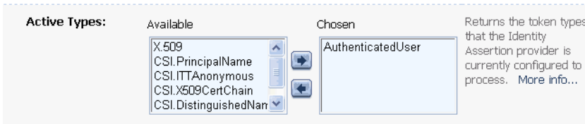
Figure 4-1 Configuring the Sample Identity Assertion Provider
