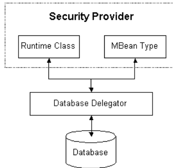
Figure 2-11 Positioning of the Database Delegator Class
