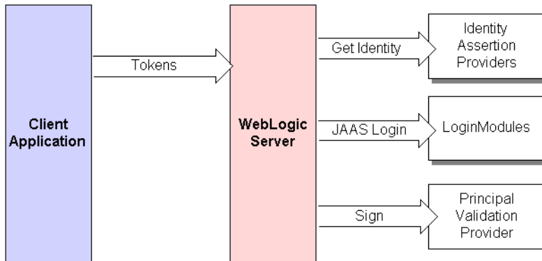
Figure 4-2 Perimeter Authentication
