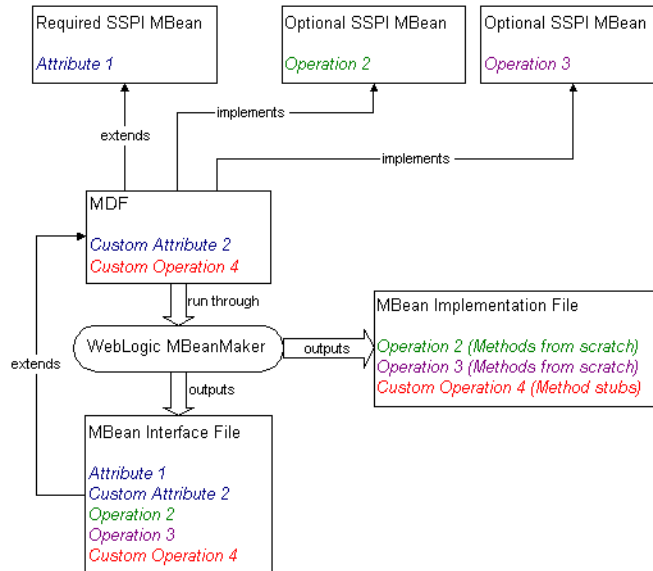
Figure 2-7 What the WebLogic MBeanMaker Provides
