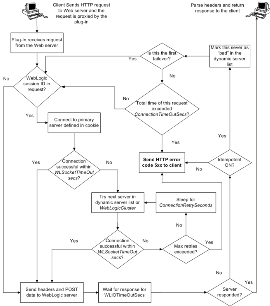
Figure 3-1 Connection Failover
