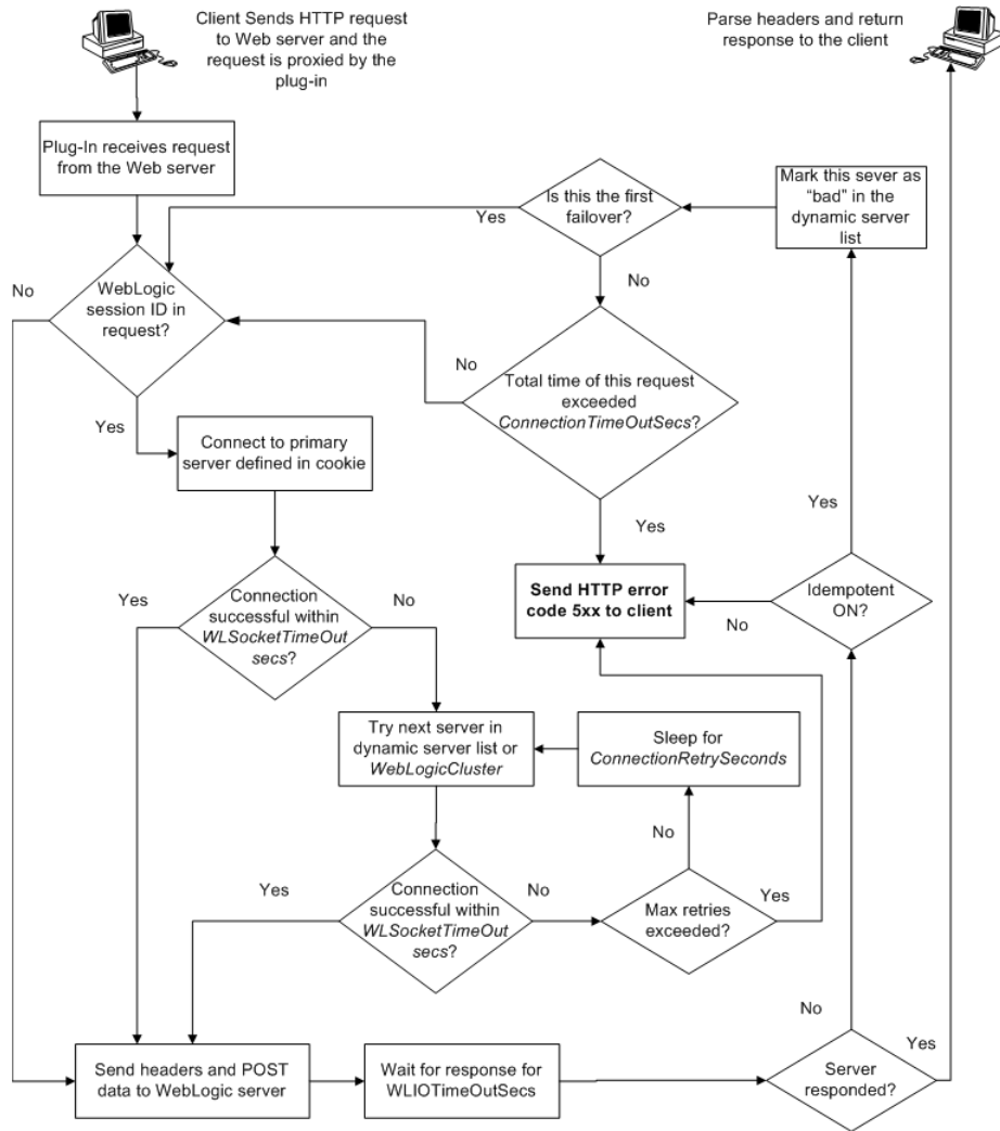
Figure 5-1 Connection Failover
