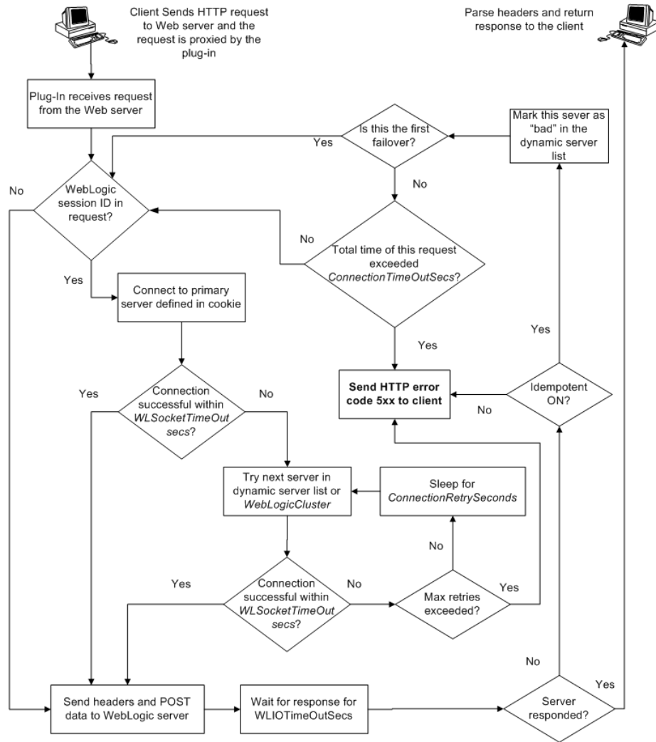
Figure 4-1 Connection Failover
