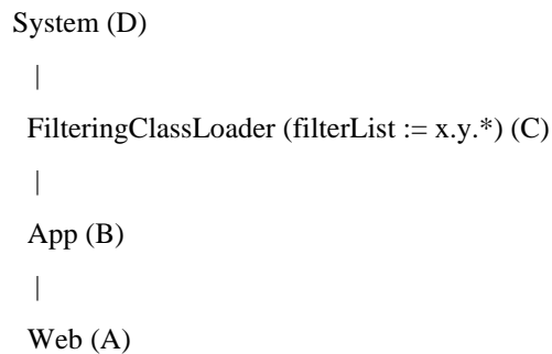
Figure 7-6 Using a Filtering Classloading Implementation
