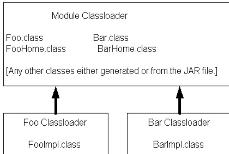
Figure 7-4 Example Classloader Hierarchy for a Single EJB Module
