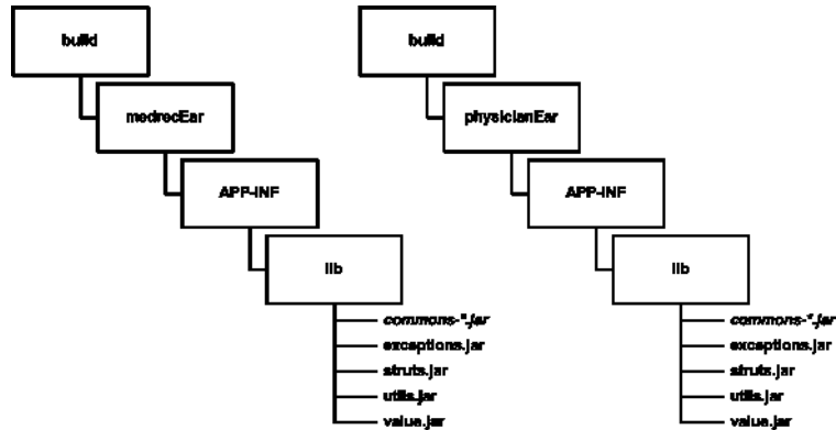
Figure 3-9 Shared JAR Files in MedRec
