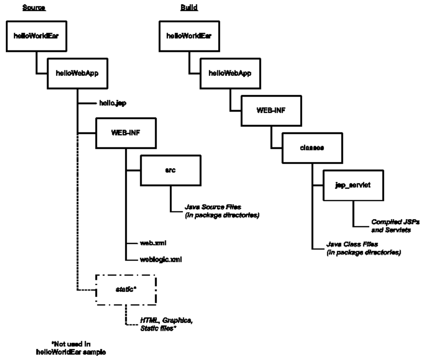
Figure 3-5 Web Application Source and Build Directories
