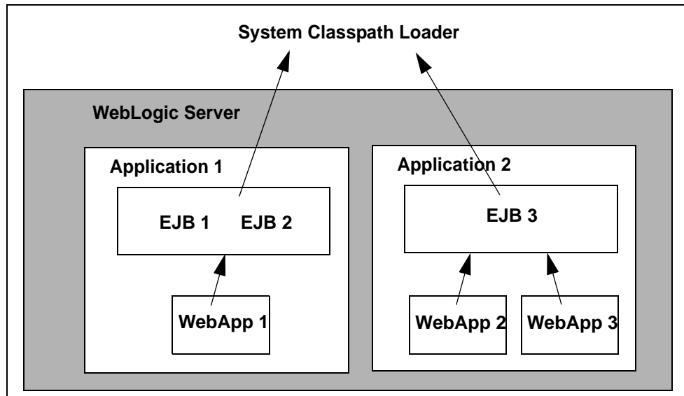
Figure 7-1 WebLogic Server Classloading
