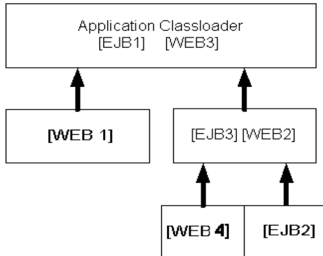
Figure 7-3 Example Classloader Hierarchy
