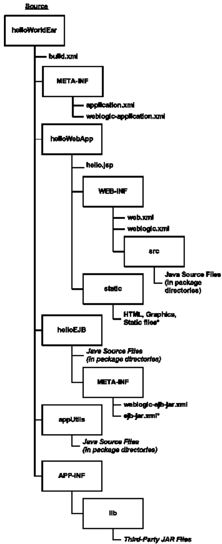
Figure 3-3 Overview of Enterprise Application Source Directory
