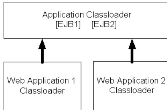
Figure 7-2 Standard Classloader Hierarchy
