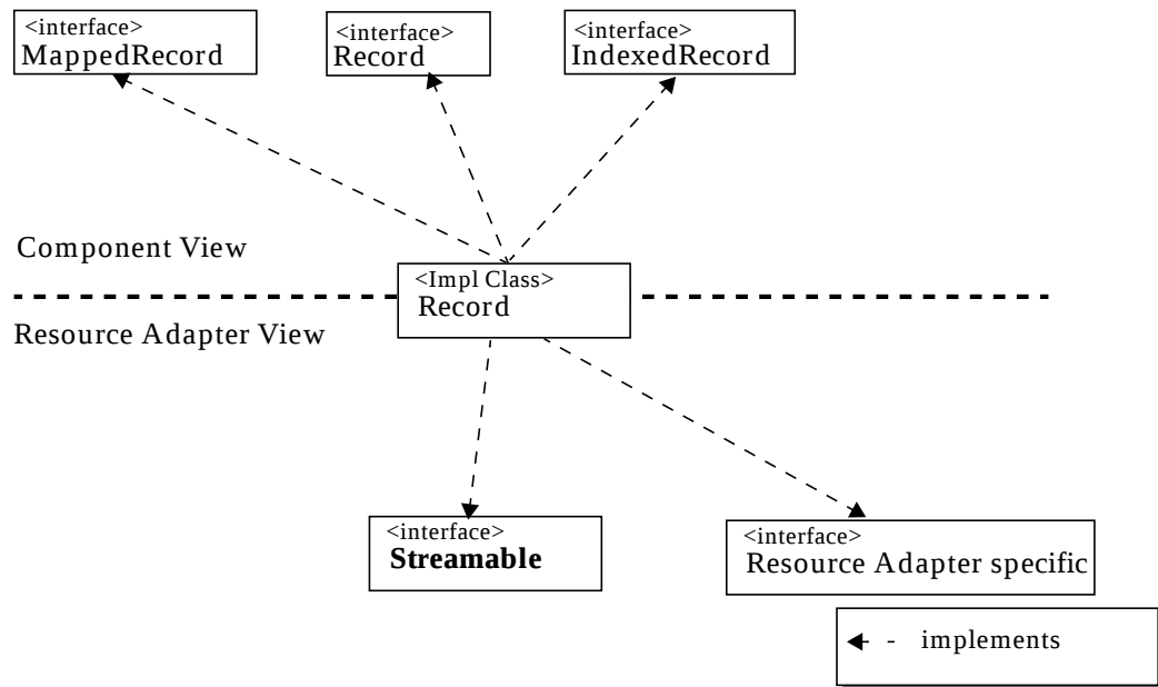
FIGURE 36.0 Streamable Interface
