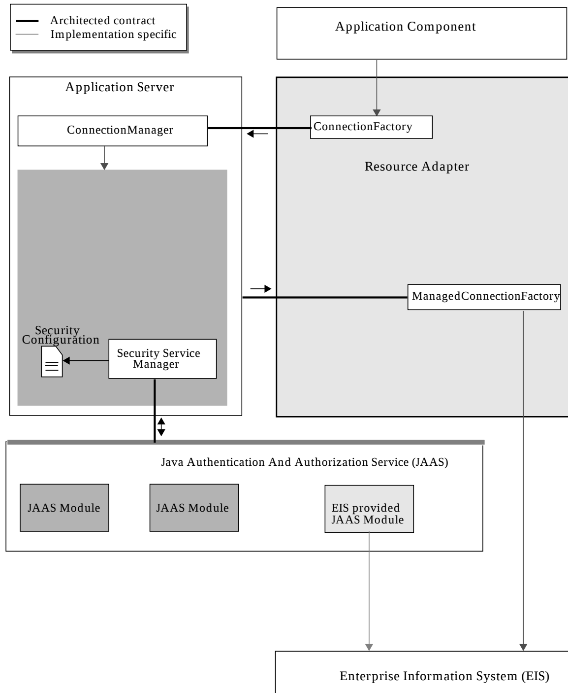
FIGURE 48.0 Security Architecture.
