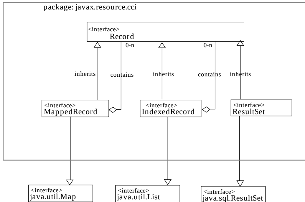
FIGURE 35.0 Component-view Contract
