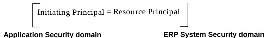
FIGURE 45.0 Principal Mapping
