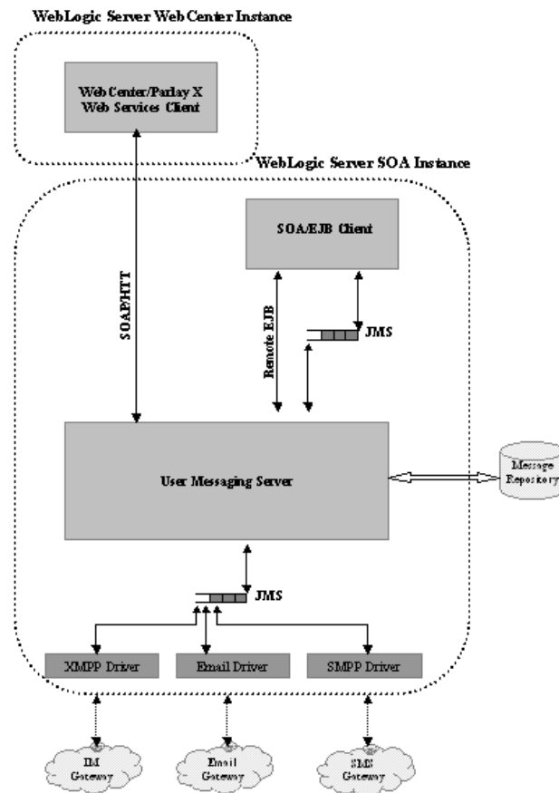
Figure 27-1 UMS architecture
