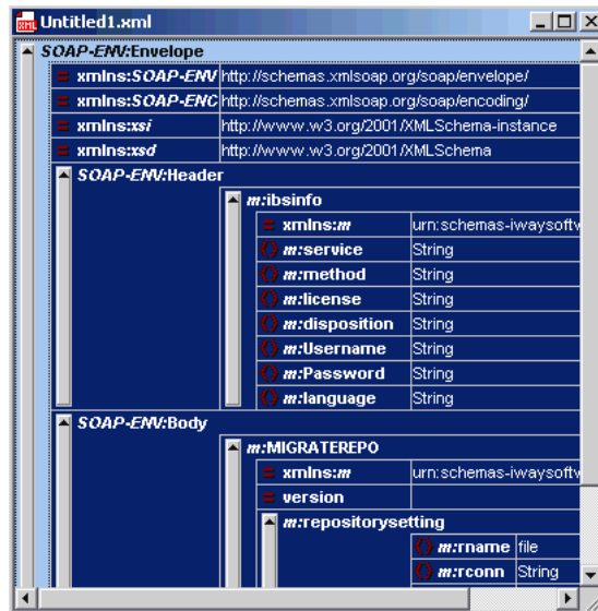
Figure 9–18 SOAP Envelope Structure
