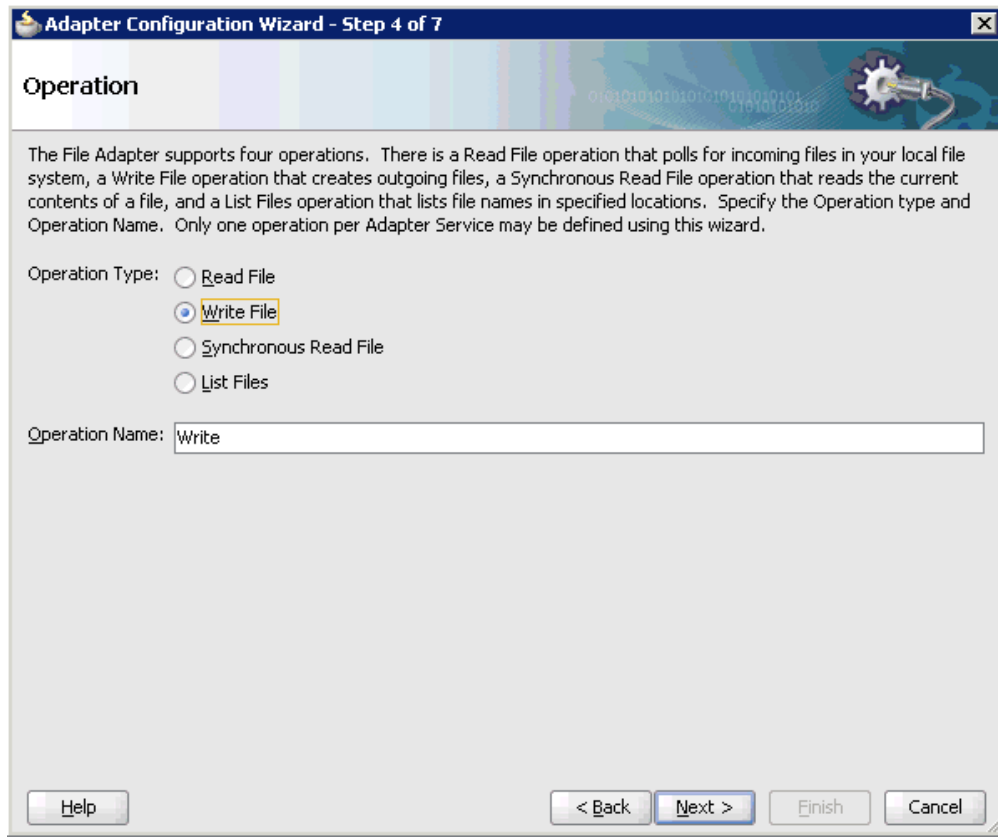
Figure 6–129 Operation Page
