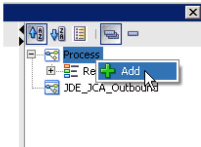
Figure 6–31 Add Option
