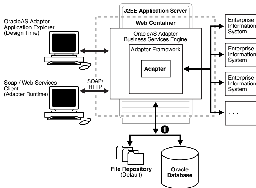
Figure 1-3 Oracle Adapter Business Services Engine (BSE) Architecture
