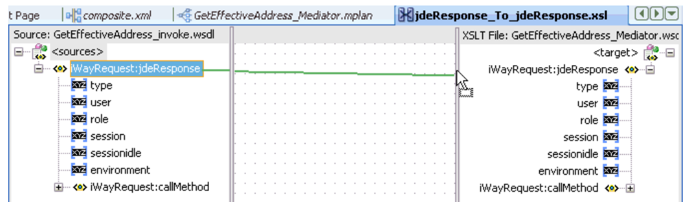
Figure 5-76 jdeResponse_To_jdeResponse.xsl Tab
