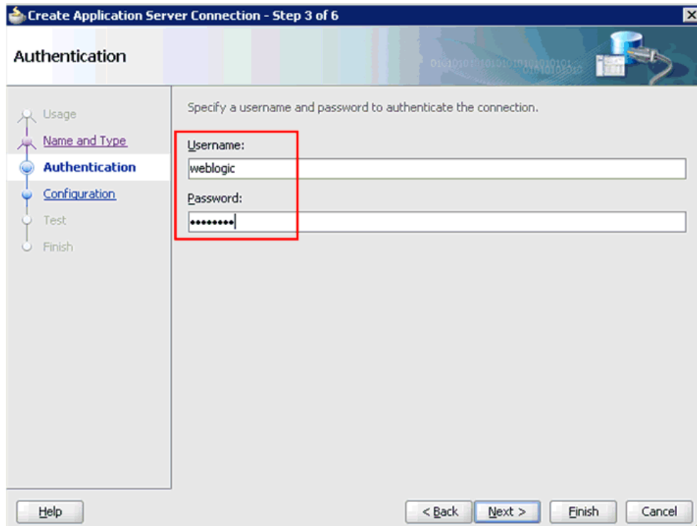
Figure 4-5 Authentication Page
