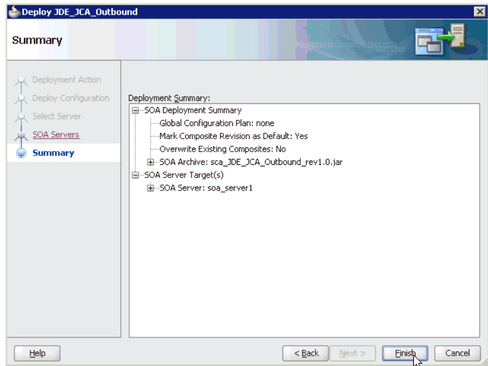
Figure 6–87 Summary Page
