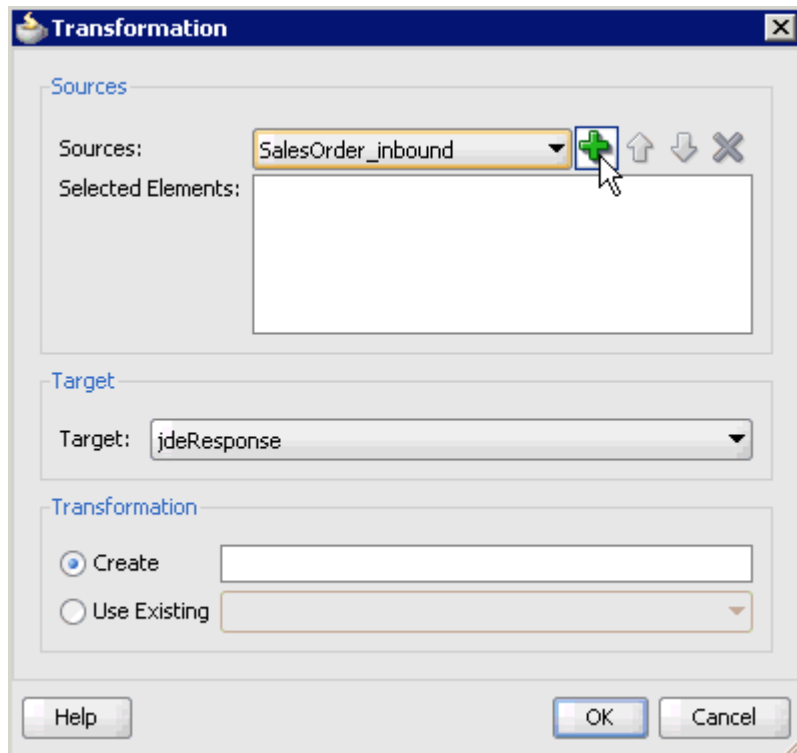
Figure 6-145 Transformation Dialog
