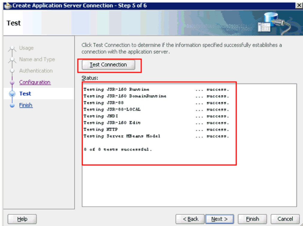
Figure 4–7 Test Page
