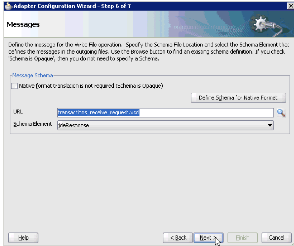
Figure 5–69 Messages Page
