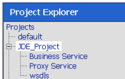
Figure 7-6 Project Explorer
