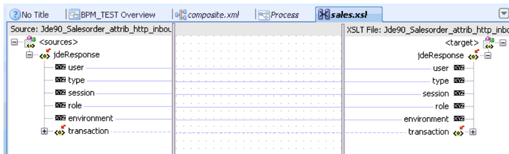
Figure 6–152 Completed Transformation
