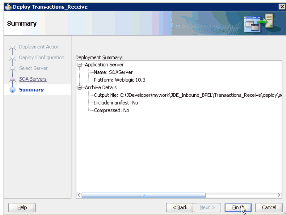
Figure 4–95 Summary Page
