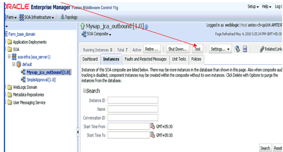
Figure 6–90 Test Button
