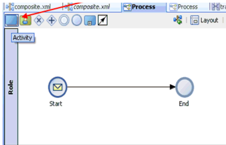
Figure 6–136 BPMN Process
