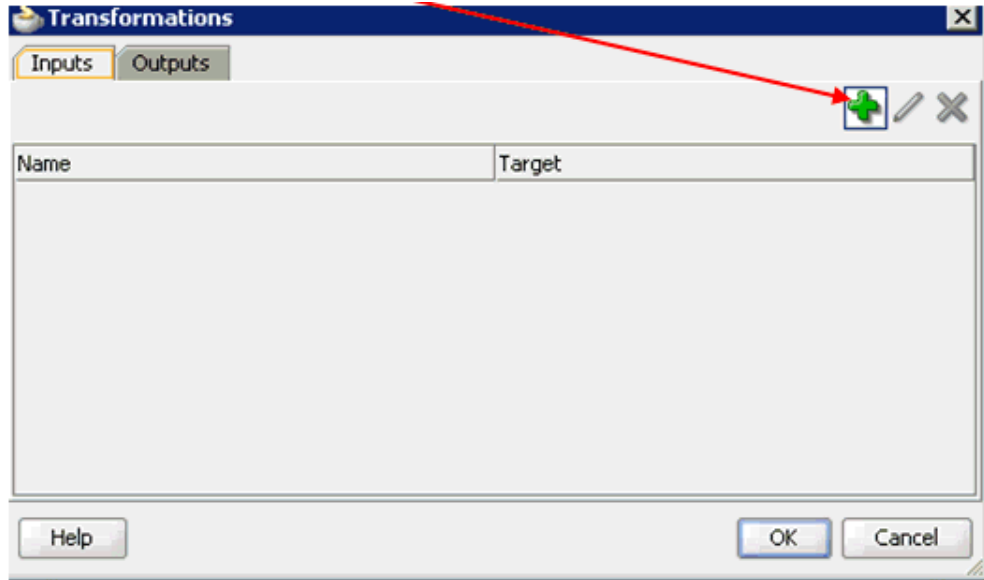
Figure 6-144 Transformations Dialog
