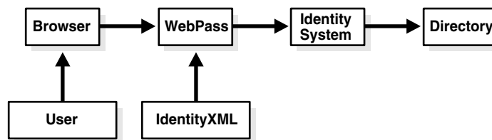
Figure 1-3 IdentityXML can Substitute for User Interaction
