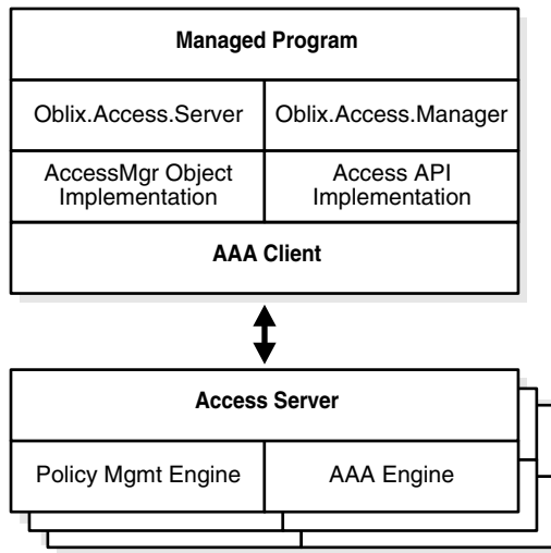
Figure 5–2 Java and C bindings for Policy Management API
