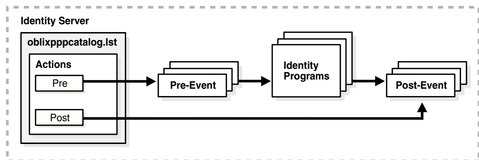
Figure 3-1 Pre-processing Event and Post-processing Event
