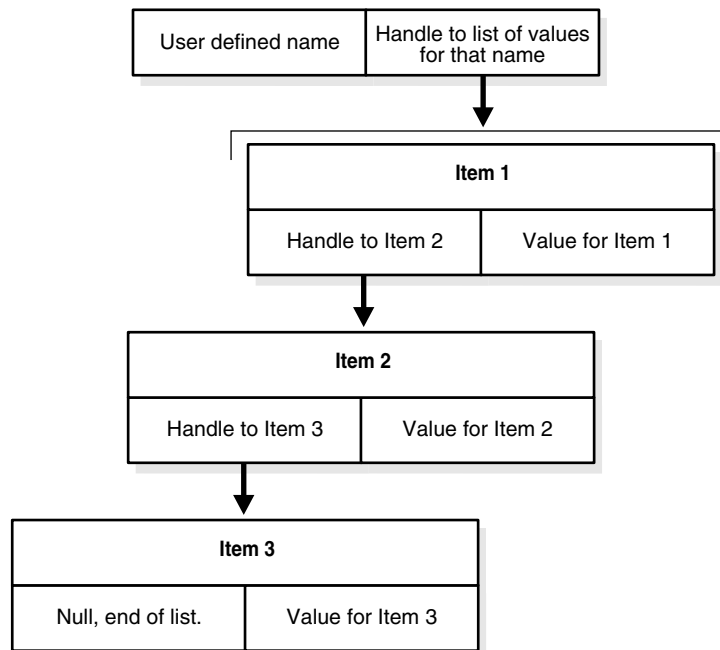
Figure 6-1 Illustration of GetDataFn
