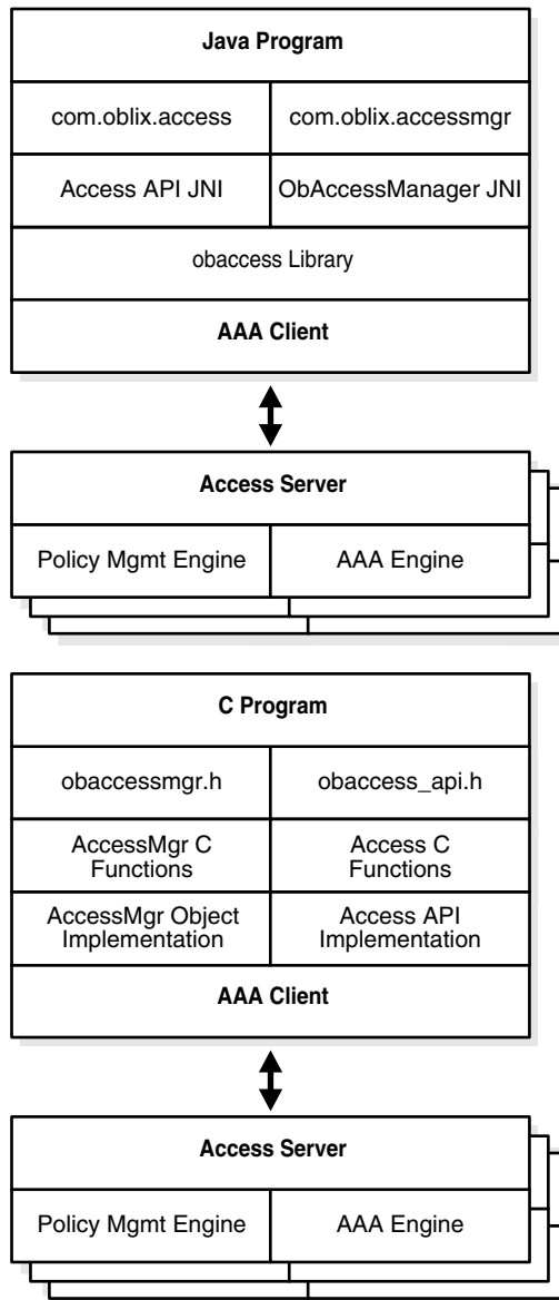
Figure 5-1 Java and C bindings for Policy Manager API
