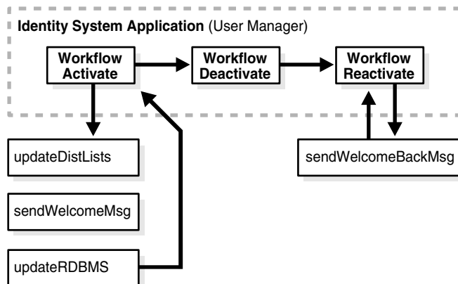
Figure 3–3 How Events are Triggered
