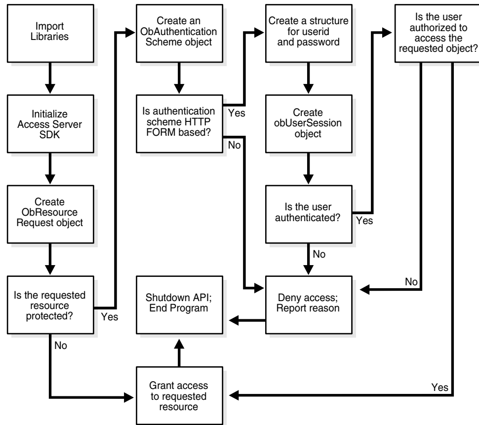
Figure 4-3 Process Flow for Form-based Applications
