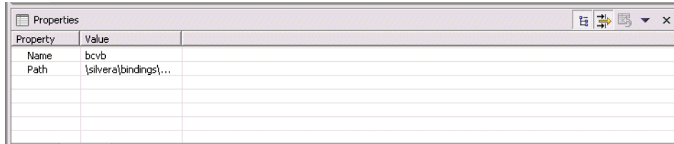
Figure 12–3 Properties View
