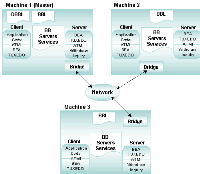
Figure 10-1 Sample of a Distributed Application
