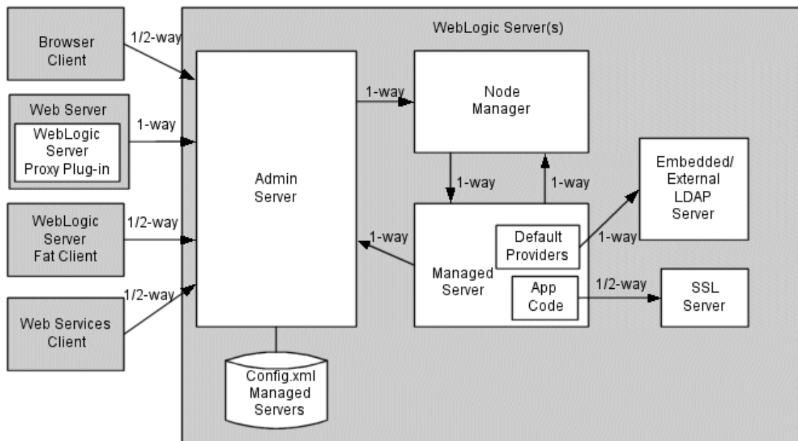
Figure 3–3 How WebLogic Server Supports SSL Connections
