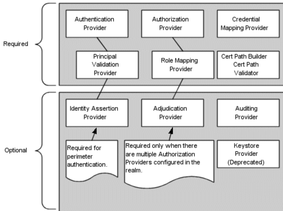
Figure 4–3 WebLogic Security Providers in a Security Realm
