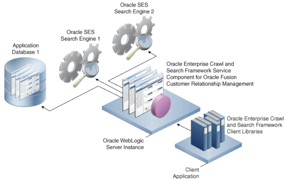
Figure 31–6 Federated Oracle SES
