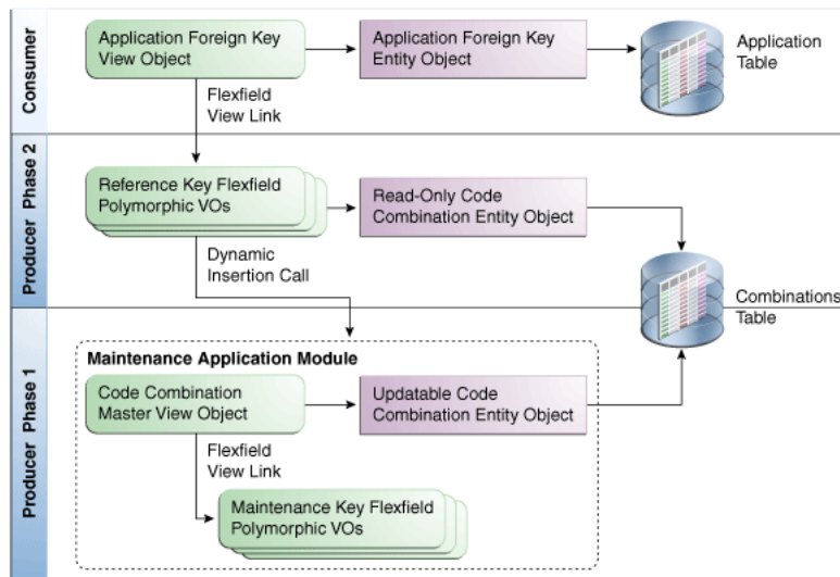
Figure 24–1 Key Flexfield Development Roles, Business Components and Supporting Artifacts
