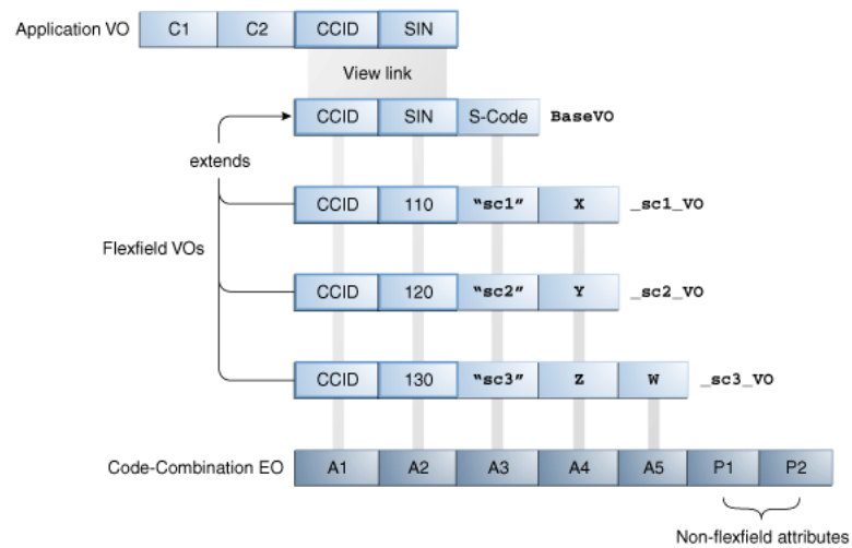
Figure 24–2 Key Flexfields Modeled as ADF Business Components
