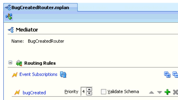
Figure 32-2 Mediator Subscription to an Event
