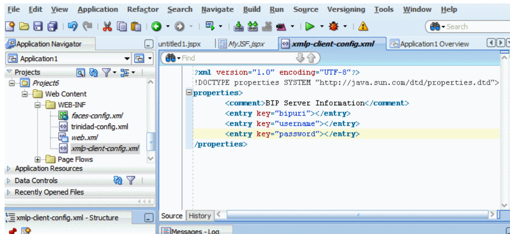
Figure 11–8 Entering the Connection Keys
