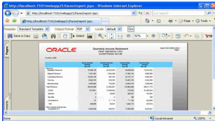
Figure 11–16 Generated Report
