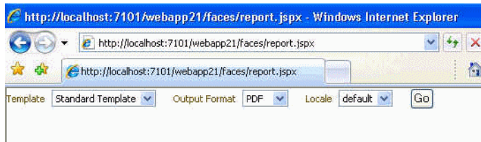
Figure 11–15 Displayed Fields
