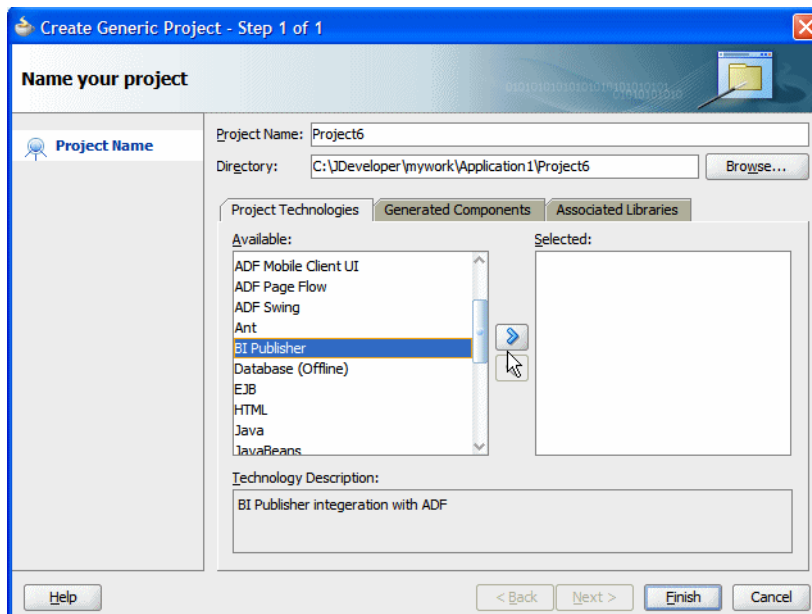
Figure 11-1 Selecting the BI Publisher Technology Scope
