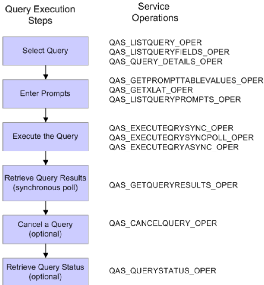
Steps to execute a query
