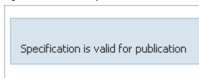
Figure 2-15: Valid Specification
