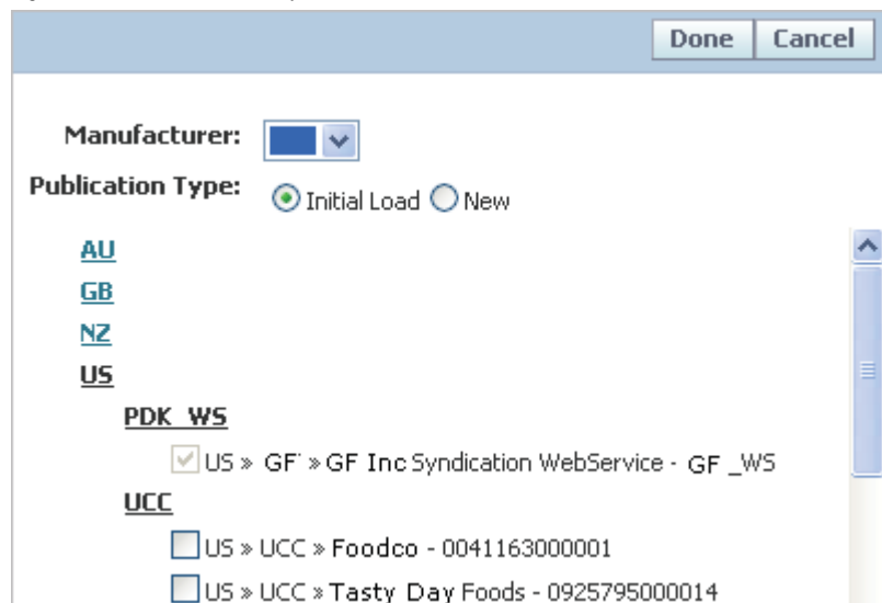
Figure 2-3: Publications requirements
