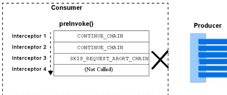
Figure 9–7 preInvoke() Chain
