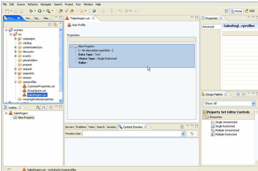
Figure 4-2 A Single Restricted Property Lets You Pick a Value From a List that You Define
