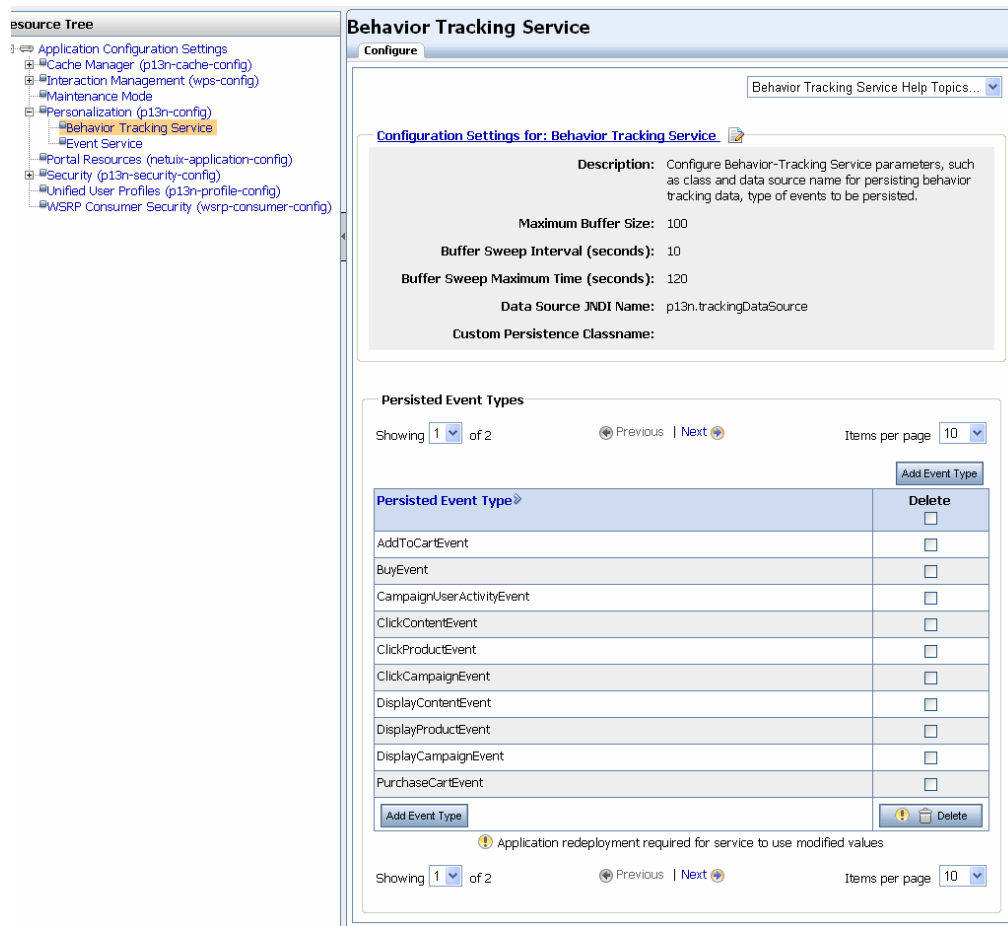
Figure 9–9 Click Add Event Type
