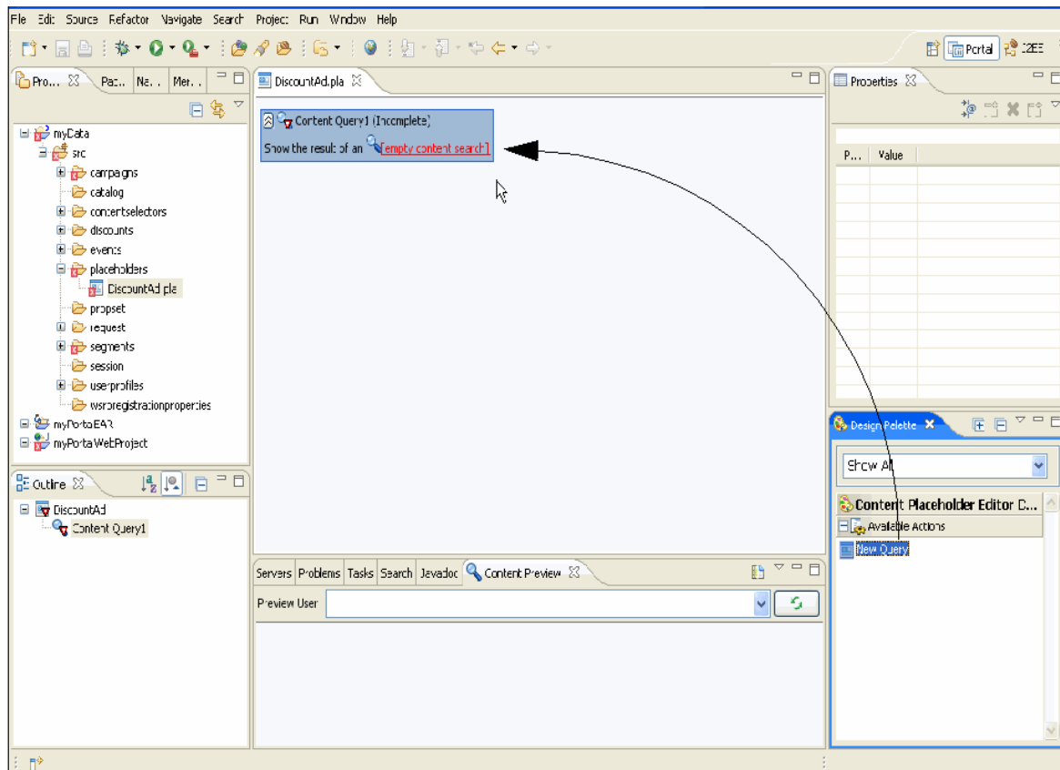
Figure 7–2 Define a Default Query by Dragging the New Query into the Placeholder Editor
