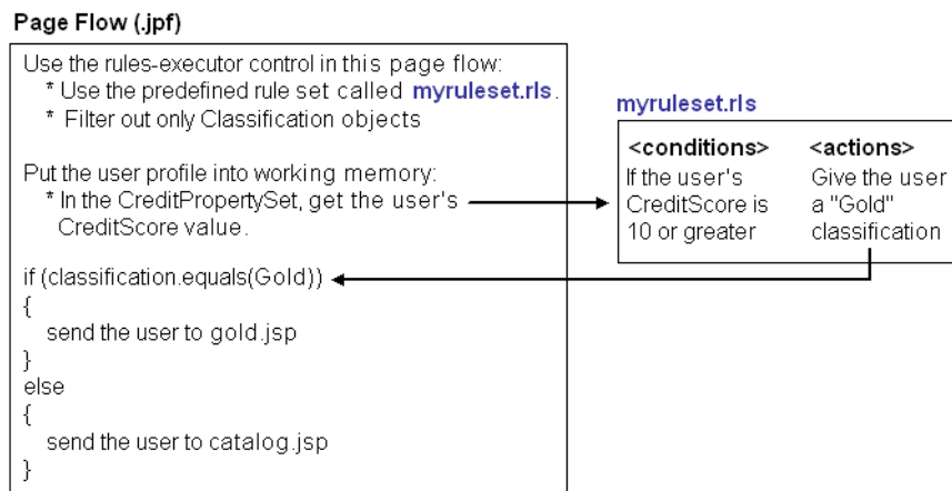
Figure 10–1 Using Rules to Control a Page Flow
