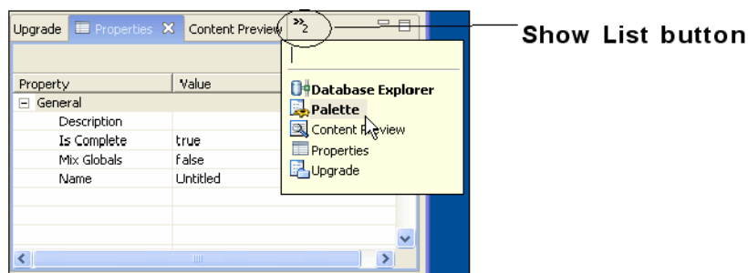
Figure 7–3 Click Show List to View Hidden Tabs
