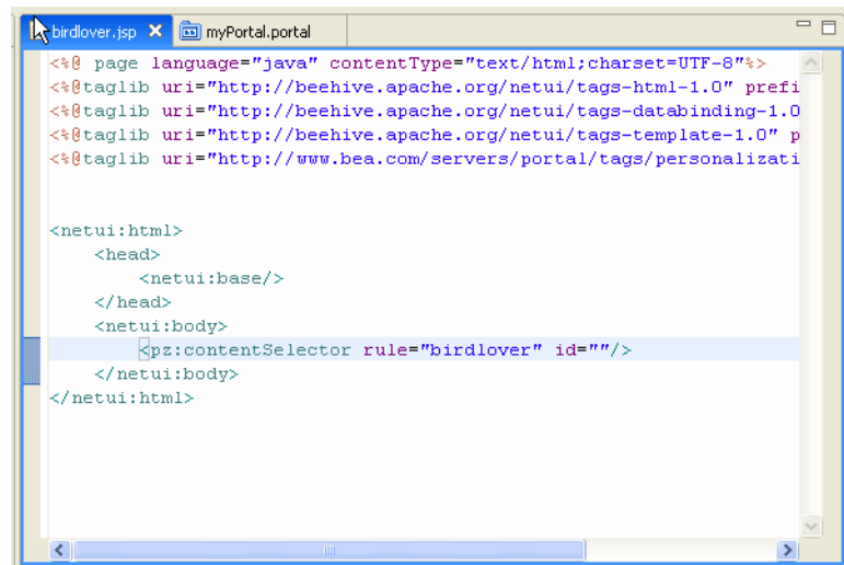
Figure 6–5 Adding a Content Selector to a JSP in Oracle Enterprise Pack for Eclipse
