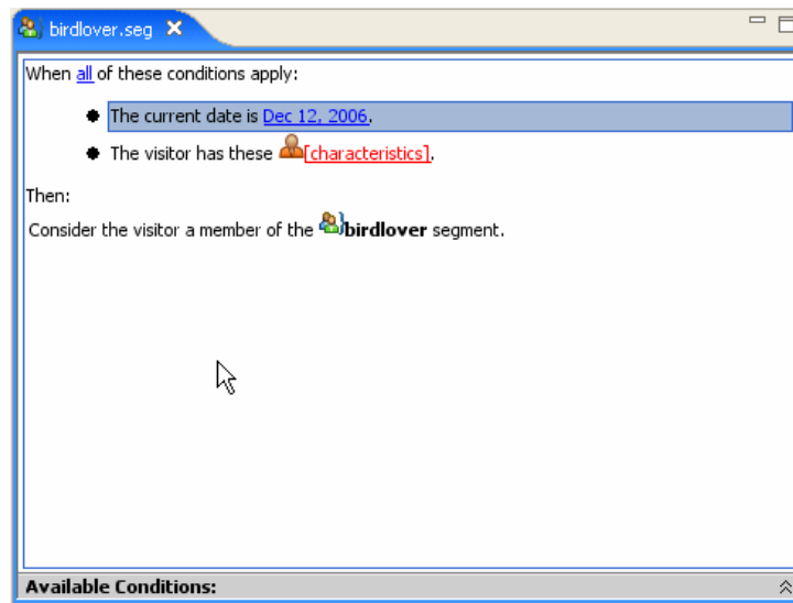
Figure 4–1 This User Segment is Called birdlover.seg
