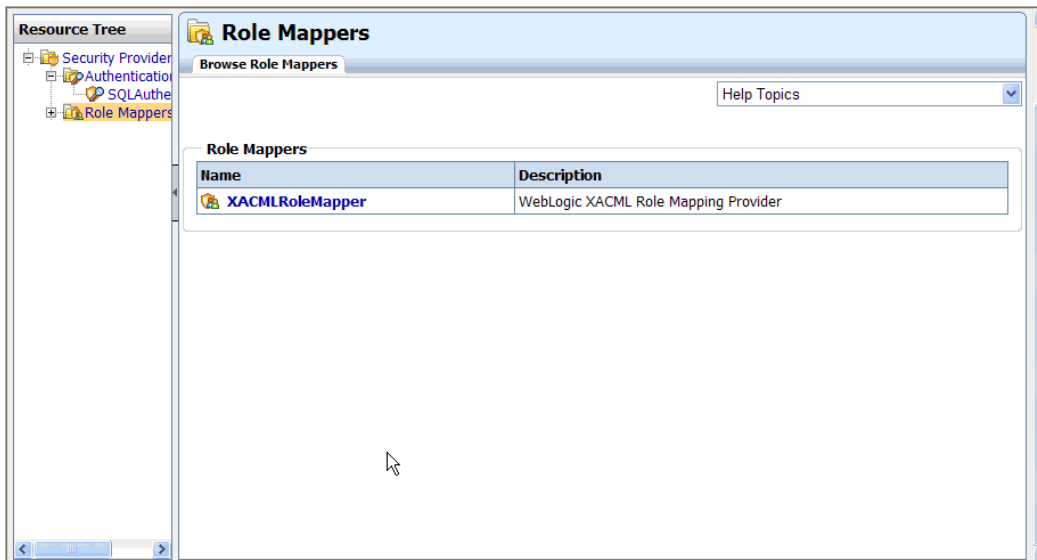
Figure 6–4 Role Mappers
