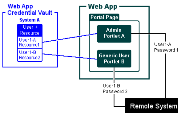
Figure 5–2 User + Resource Credential Vault
