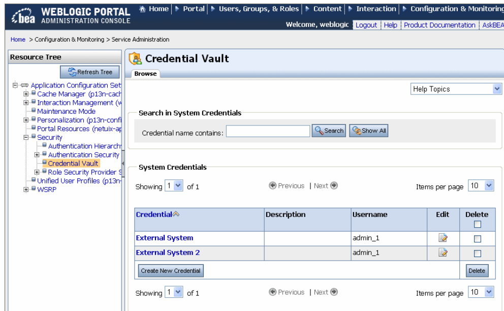
Figure 5–4 Credential Vault
