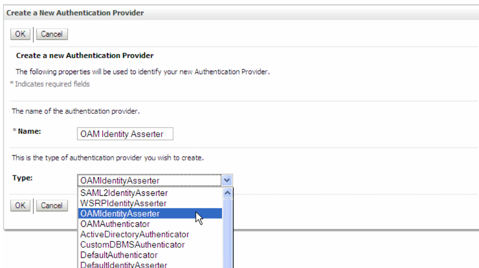
Figure 6–7 Selecting OAMIdentityAsserter
