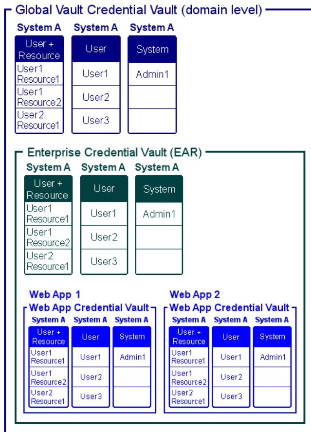
Figure 5–3 Credential Vaults
