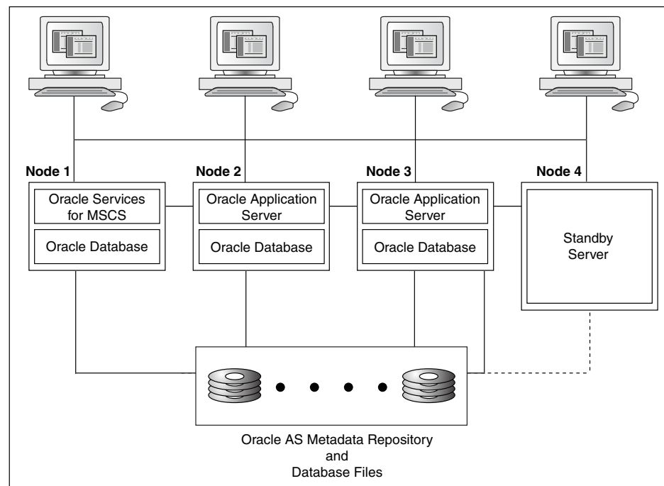
Figure 3–2 Active/Passive (Standby) Four-Node Configuration
