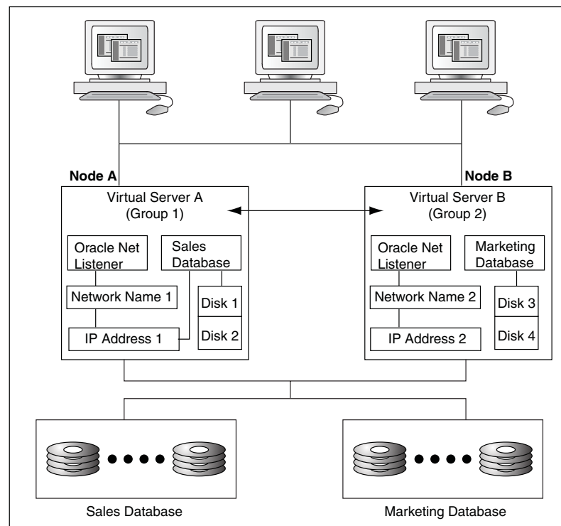
Figure 2–5 Accessing Cluster Resources Through a Virtual Server
