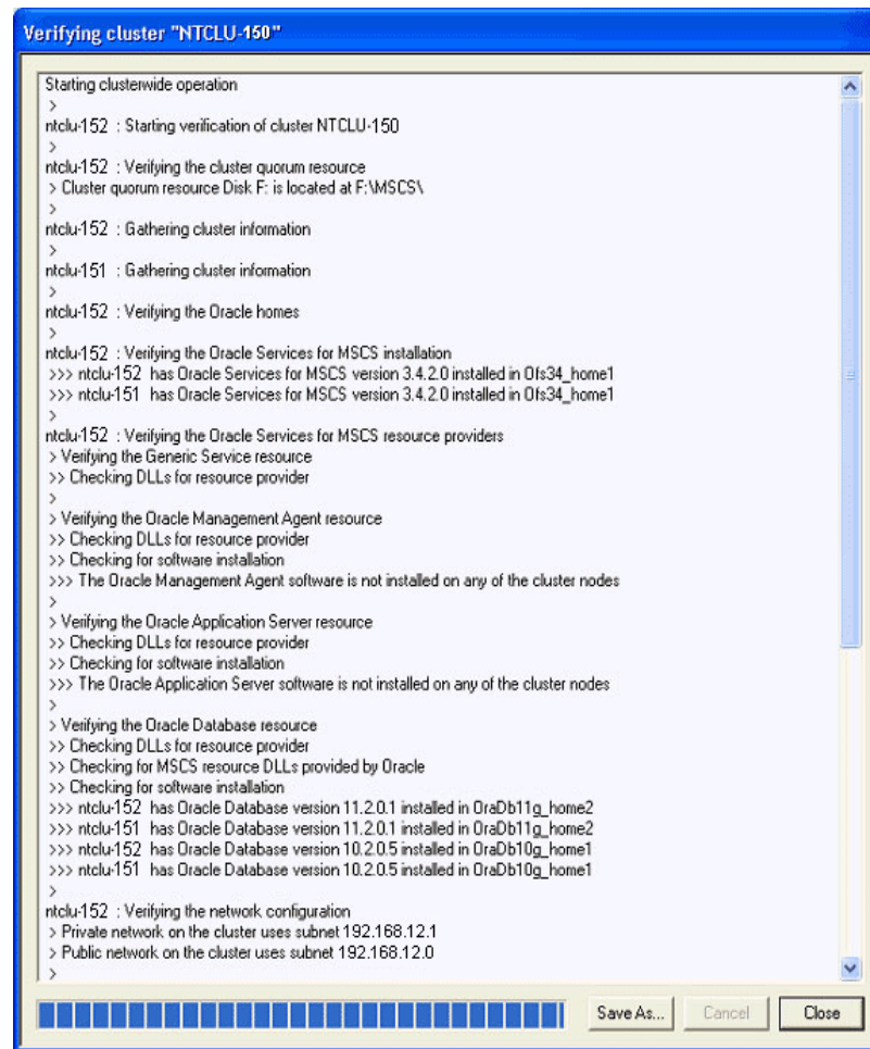
Figure 6–2 Clusterwide Operation Window for Verify Cluster
