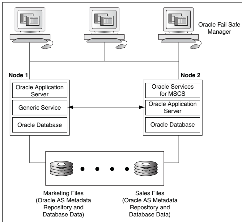
Figure 3–3 Active/Active Configuration
