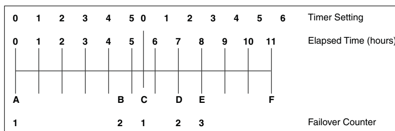
Figure 2–12 Failover Threshold and Failover Period Timeline
