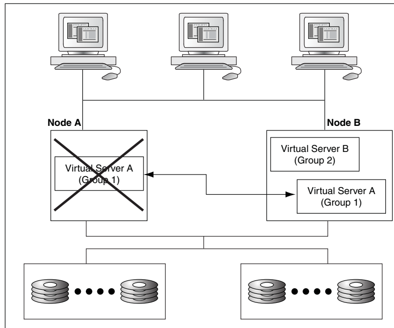
Figure 2-7 Resource Failover
