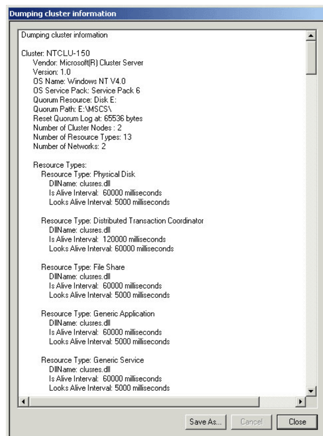
Figure 6–6 Dump Cluster Clusterwide Operation
