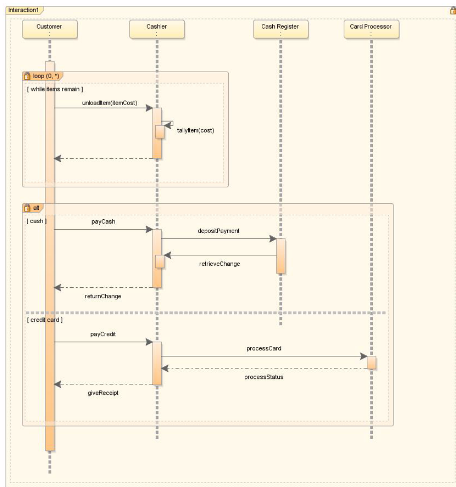
Figure 22–30 Typical Sequence Diagram with Combined Fragments
