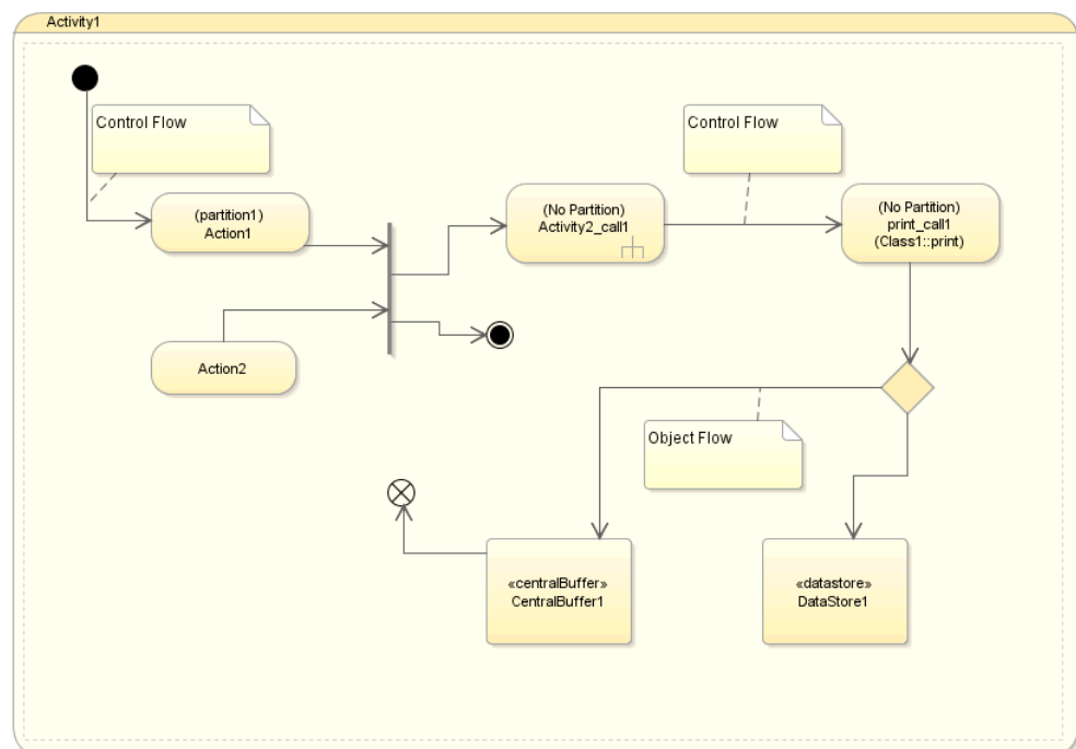
Figure 22–26 Sample Activity Diagram Showing Elements
