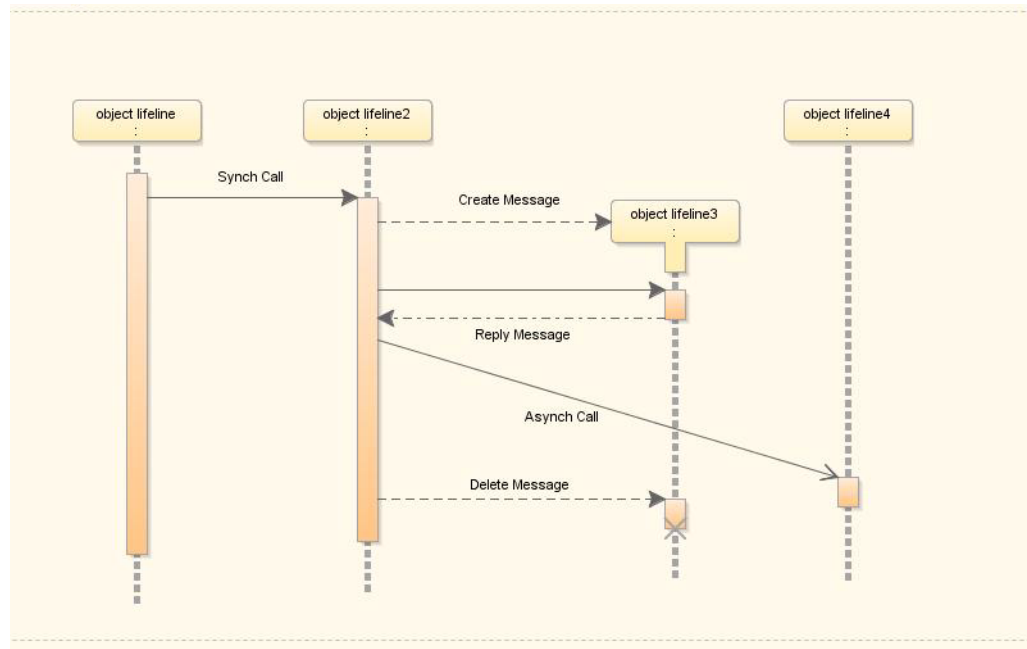
Figure 22–28 Typical Sequence Diagram Example
