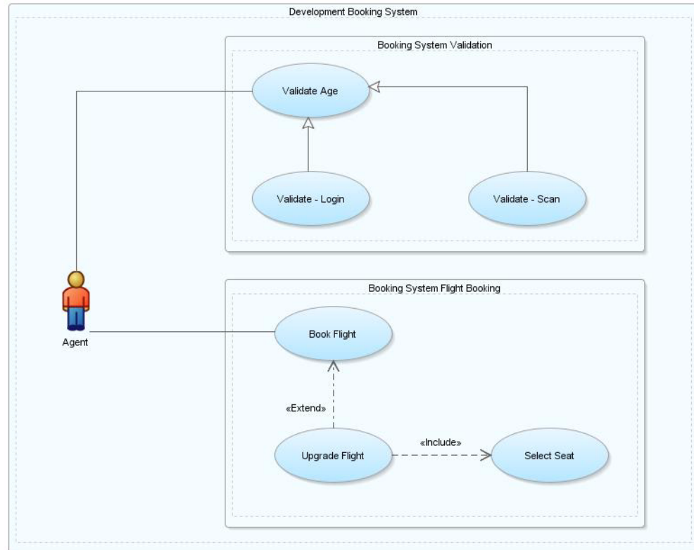
Figure 22–32 Typical Use Case Diagram
