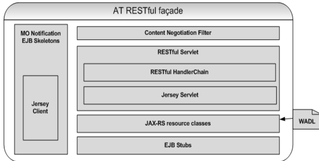
Figure 2–1 RESTful Facade
