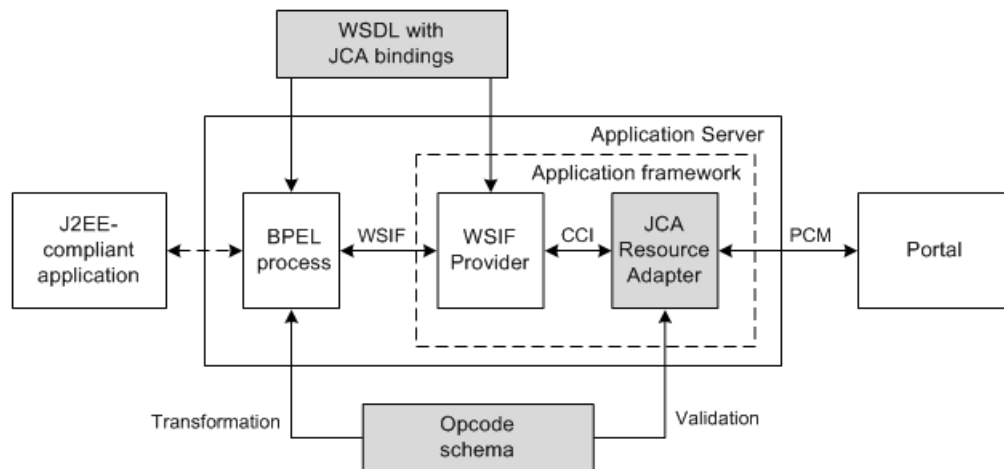
Figure 1–1 JCA Resource Adapter Architecture
