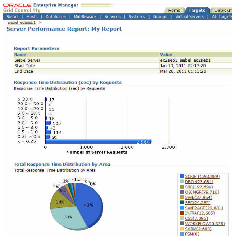
Figure 6–3 Server Performance Report - Example 1
