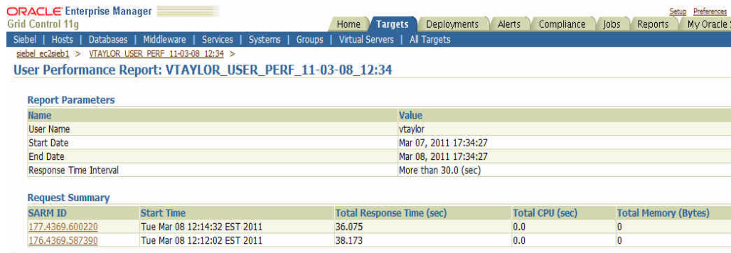
Figure 6–7 User Performance Report - Example 2
