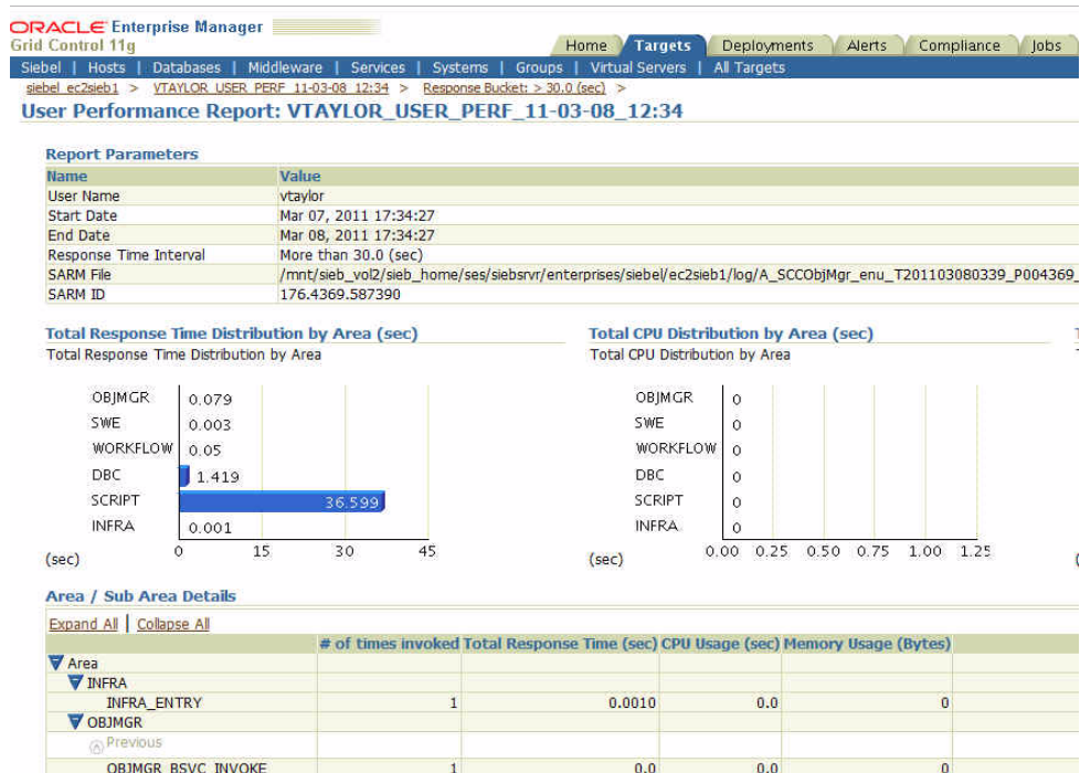
Figure 6–8 User Performance Report - Example 3
