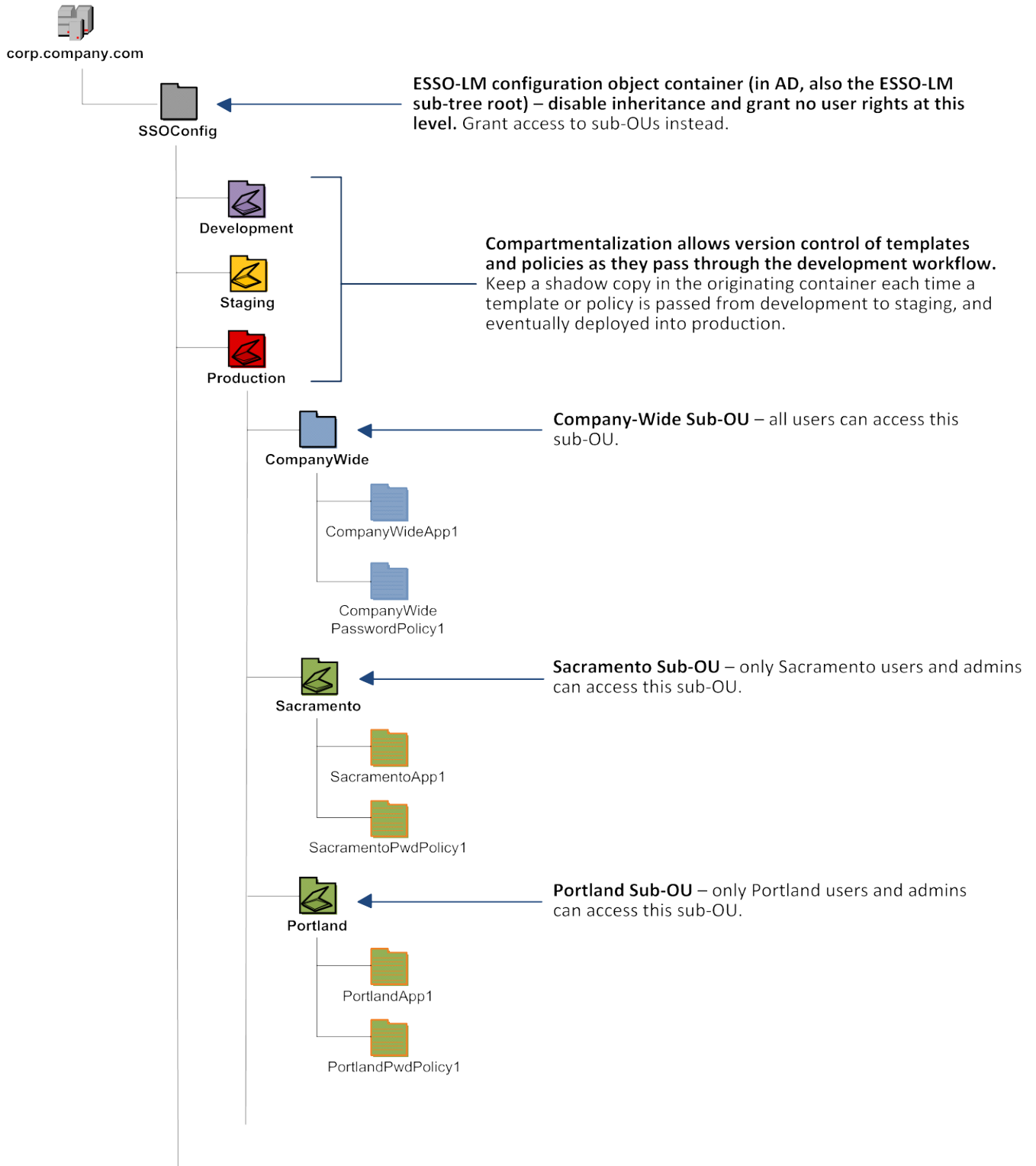
Figure 2 Recommended ESSO-LM sub-tree design
