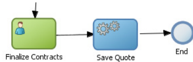
Figure 6–18 The Service Task within the Sales Quote Example Process
