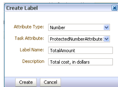
Figure 26–57 Create Label Dialog
