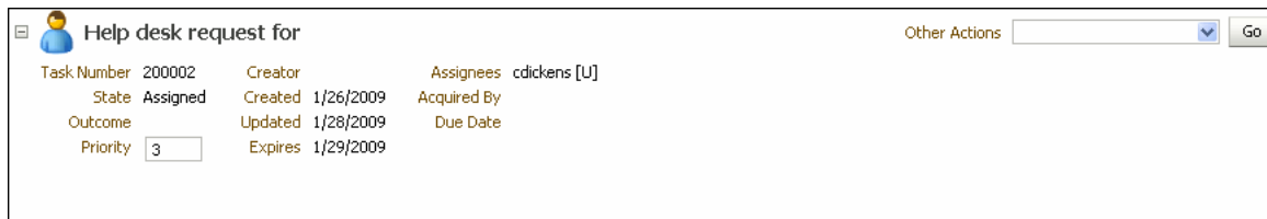
Figure 26–51 Header
