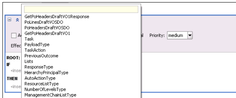
Figure 26–39 ROOT Options
