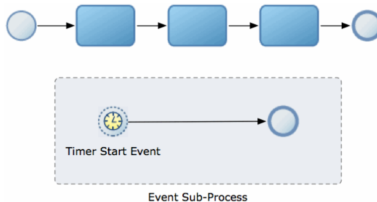
Figure 18–6
