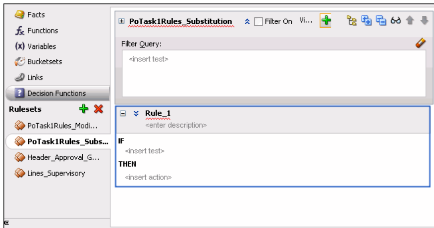
Figure 26–37 Rule-Definition Section
