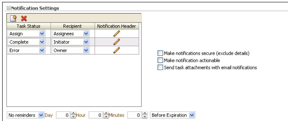
Figure 26–81 Notification Settings
