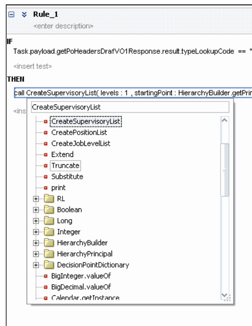
Figure 26–33 Rule Functions
