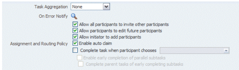
Figure 26–79 Routing Settings
