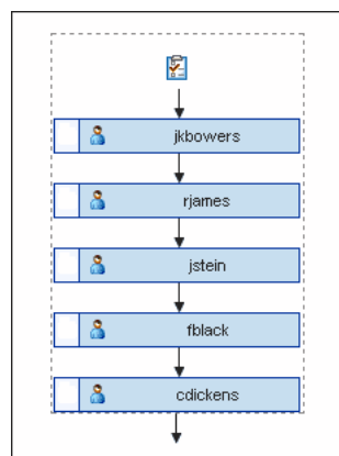
Figure 26–68 Before Move
