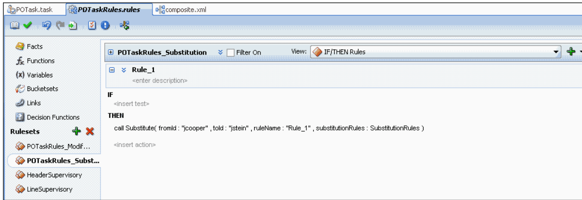
Figure 26–32 Sample Approver-Substitution Action
