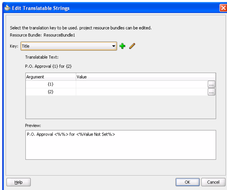
Figure 26–7 New Key Added
