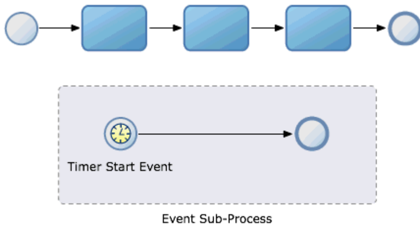
Figure 18–4 Process Deadline
