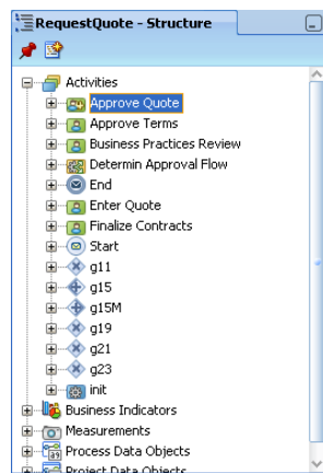
Figure 3–11 Structure View
