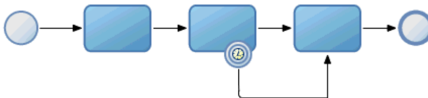
Figure 18–3 Activity Deadline
