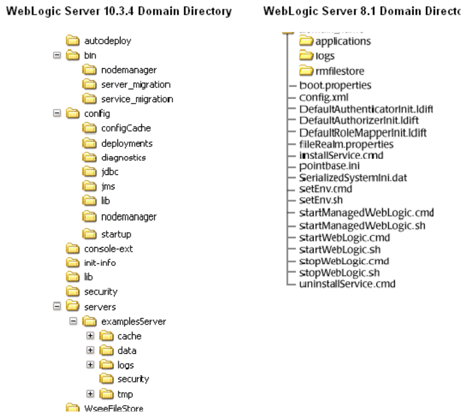
Figure C-1 WebLogic Server 10.3.4 and WebLogic Server 8.1 Directory Structures
