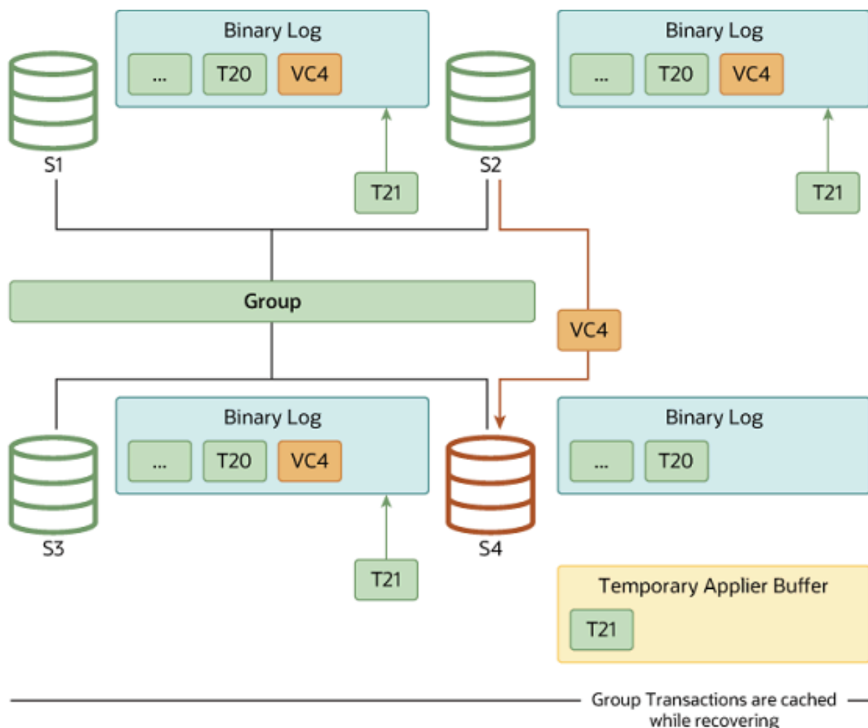
Figure 20.11 Queued Transactions
