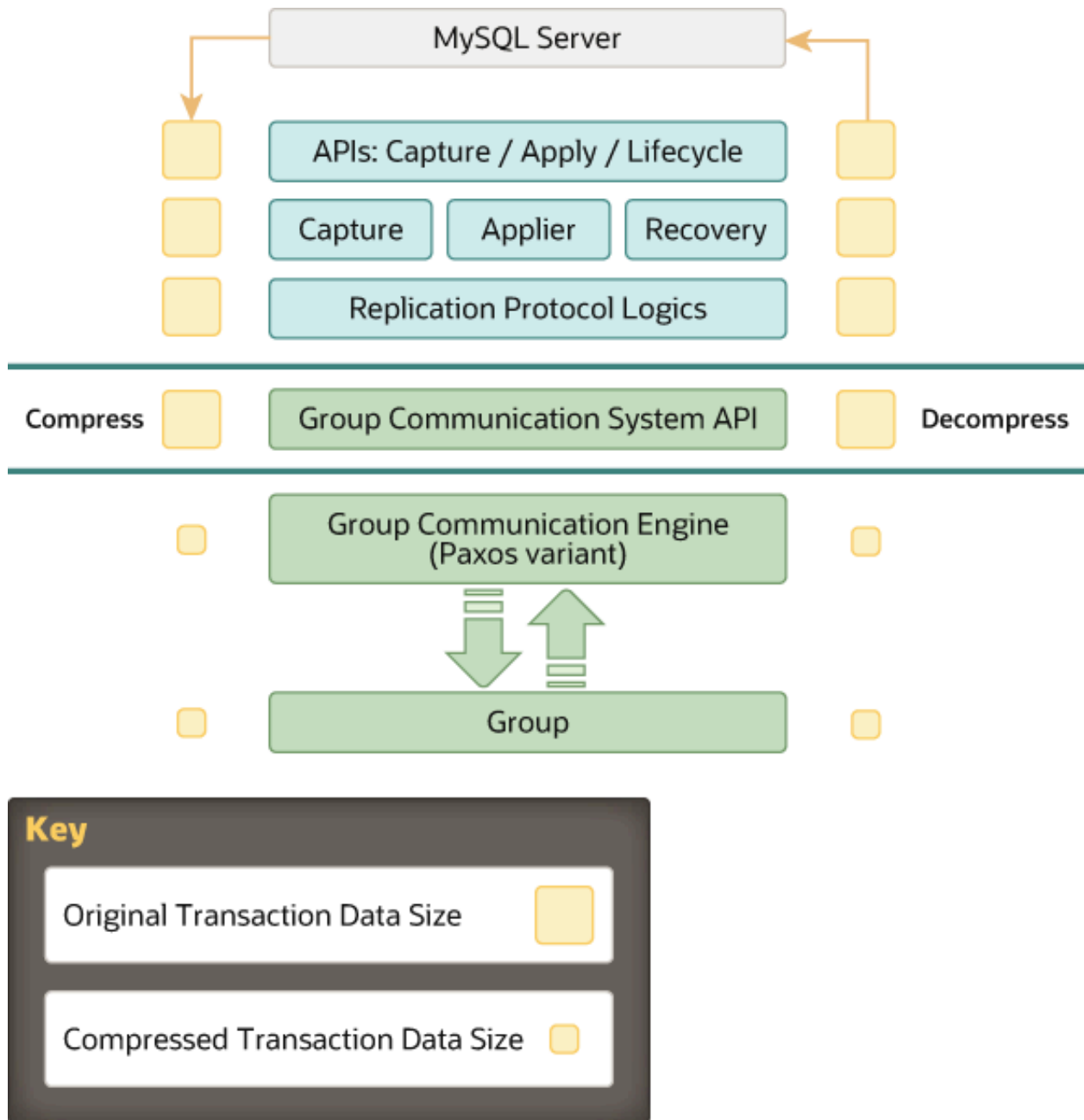
Figure 20.13 Compression Support
