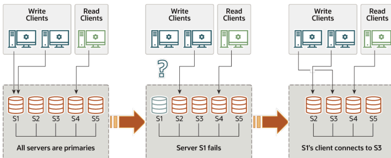
Figure 20.5 Client Failover
