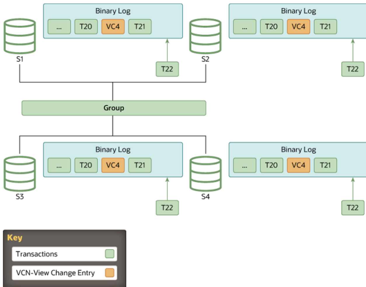
Figure 20.12 Instance Online
