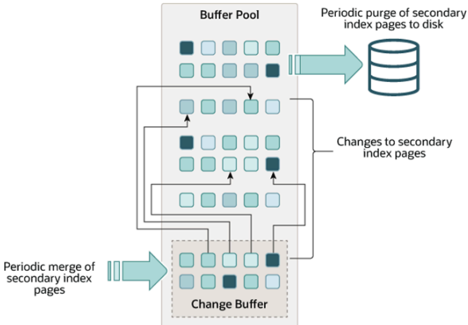
Figure 17.3 Change Buffer
