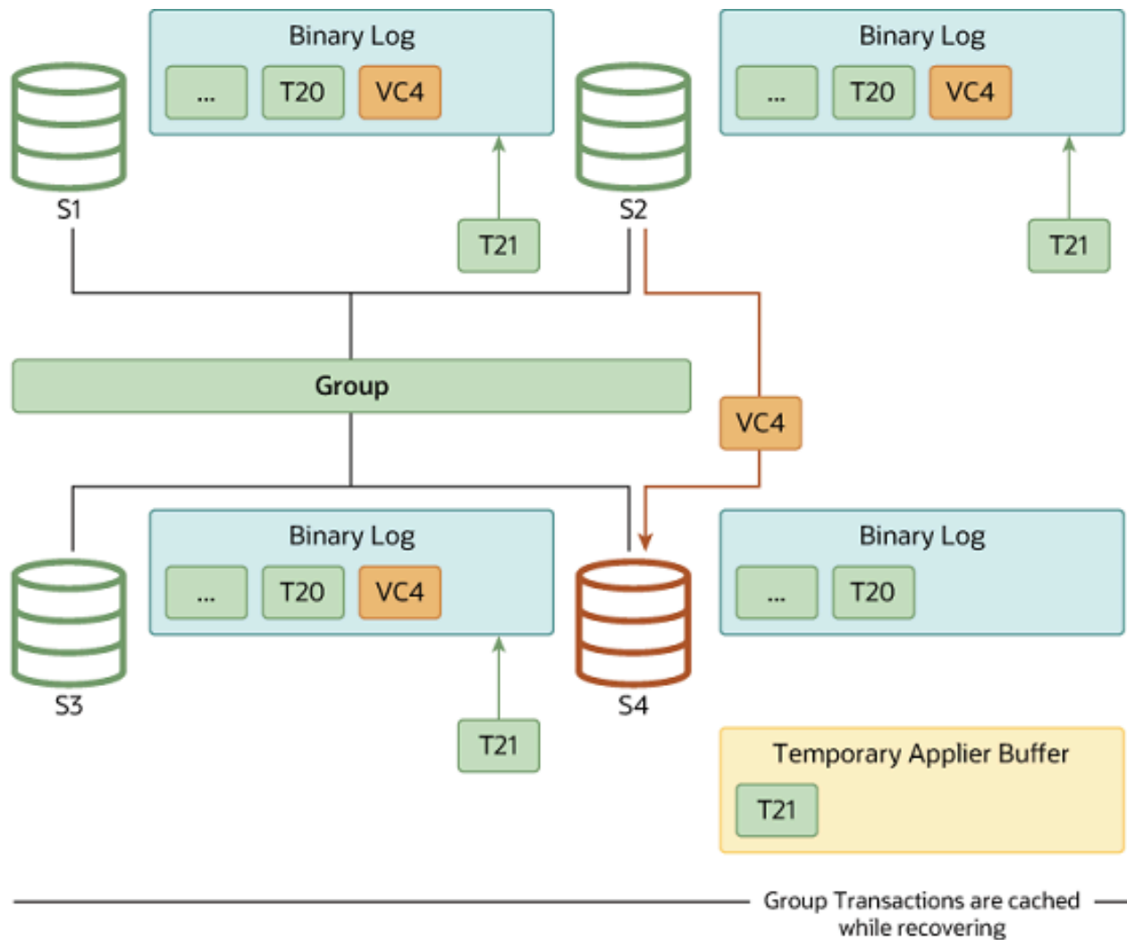
Figure 20.11 Queued Transactions
