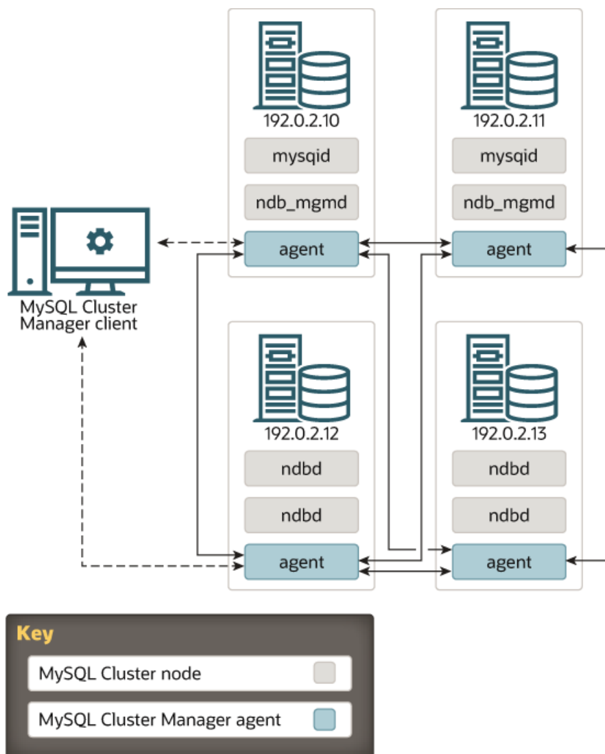
Figure 1.1 MySQL Cluster Manager Deployment
