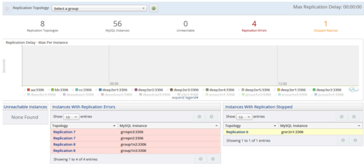
Figure 27.1 Replication Overview
