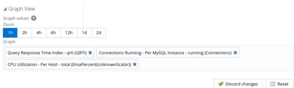
Figure 31.8 Graph View
