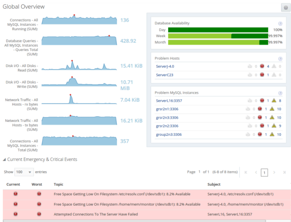
Figure 24.1 Global Overview
