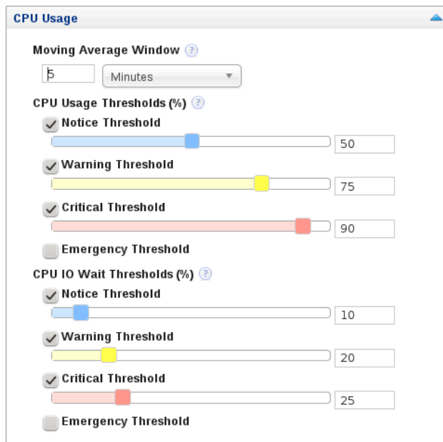
Figure 20.4 CPU Usage
