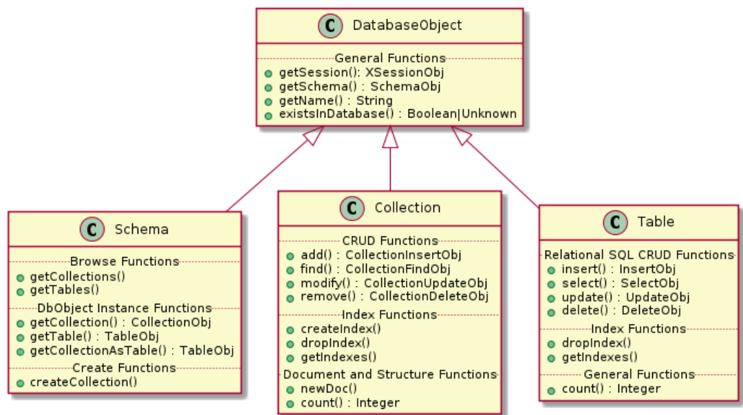
Figure 3.1 Database Object - Class Diagram
