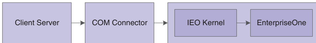
Figure A–1 COM Connector Architecture for Classic Events (Software releases prior to JD Edwards EnterpriseOne Tools 8.94)
