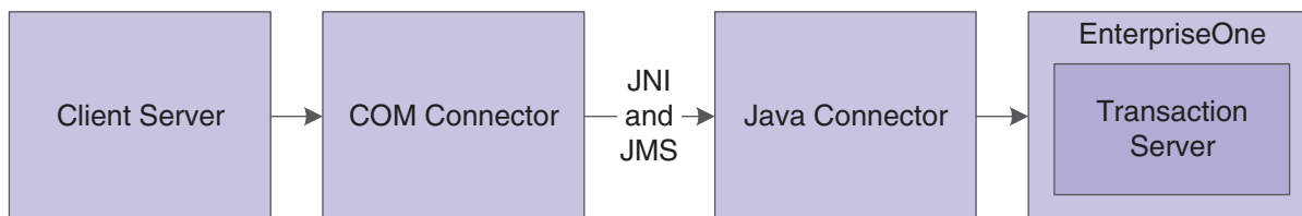
Figure 6–1 COM connector architecture-guaranteed event delivery for JD Edwards EnterpriseOne Tools release 8.94
