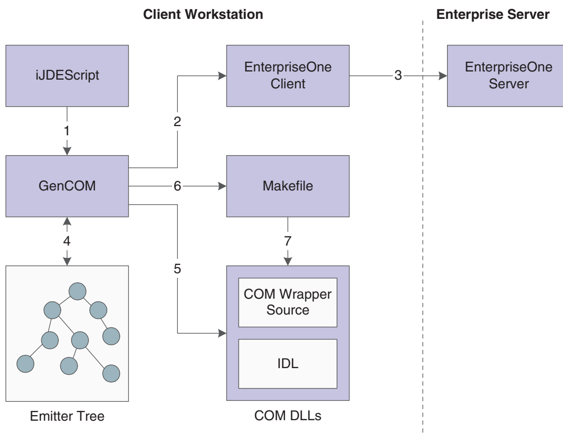
Figure 3–2 GenCOM process
