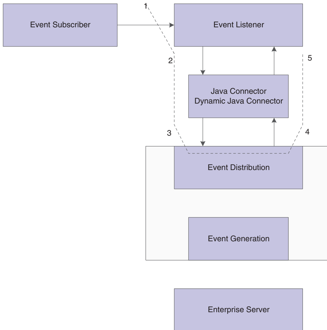
Figure B–1 Subscription and notification process
