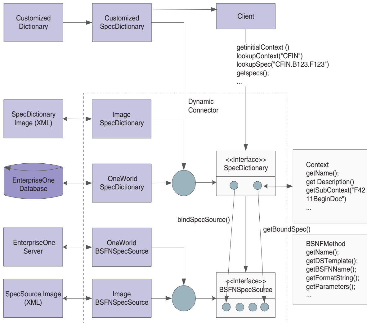
Figure 9–2 Relationship between SpecDictionary and BSFNSpecSource
