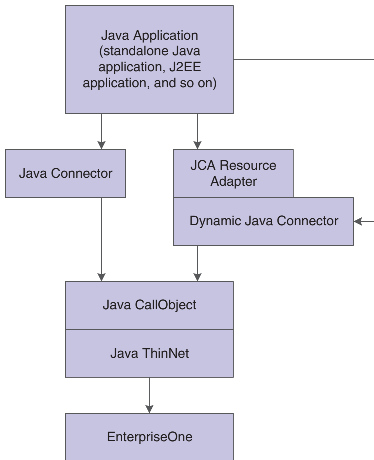
Figure 8–1 Java Application interaction with JD Edwards EnterpriseOne
