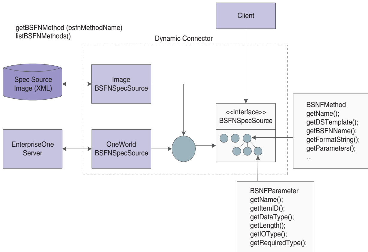
Figure 9–1 Relationships among BSFNSpecSource, BSFNMethod, and BSFNParameter
