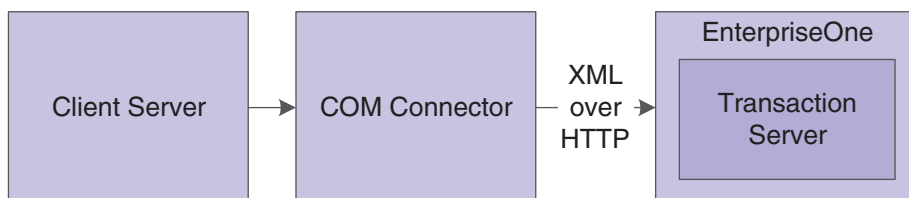
Figure 6–2 COM connector architecture-guaranteed event delivery for JD Edwards EnterpriseOne Tools release 8.95 and later Tools releases
