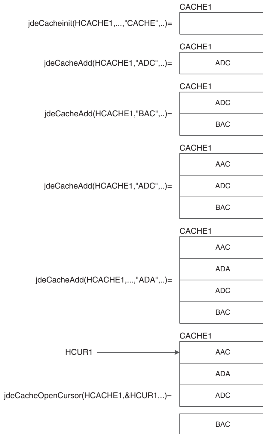
Figure 2-1 Example of JDECACHE cache and data set creation
