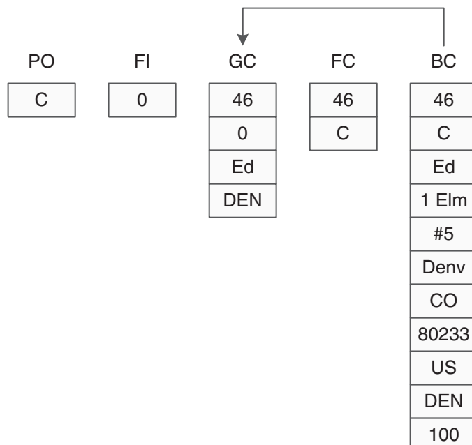
Figure 2–6 Content of runtime structures when first record is read
