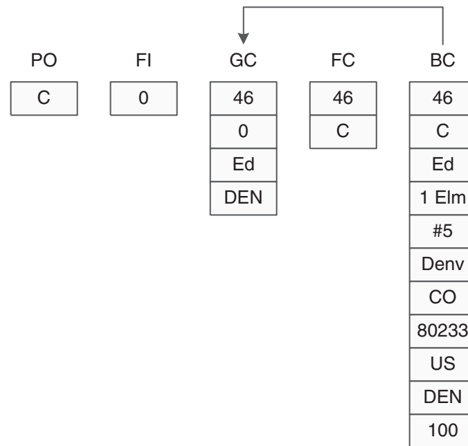
Figure 2–4 Content of runtime structures when first record read
