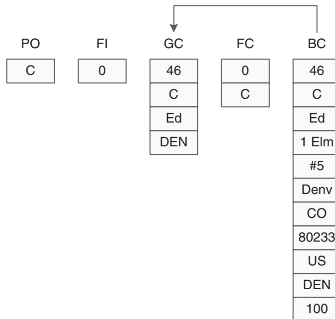
Figure 2-7 Content of runtime structures before Write Grid Line-Before fires
