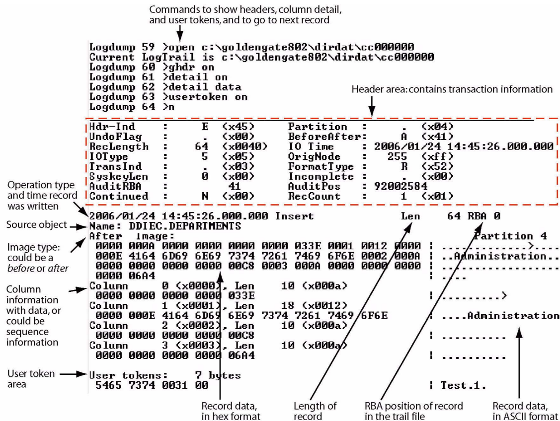
Figure 9 Sample trail record as viewed in Logdump on a Windows system
