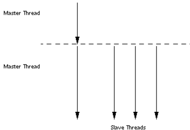
FIGURE 3-1 Master and Slave Threads
