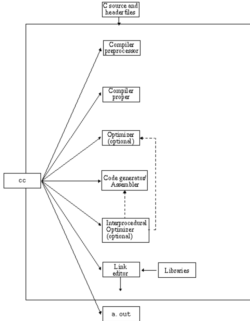
FIGURE 1-1 Organization of the C Compilation System
