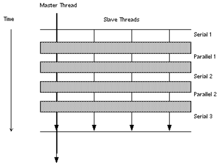
FIGURE 3-2 Parallel Execution of a Loop
