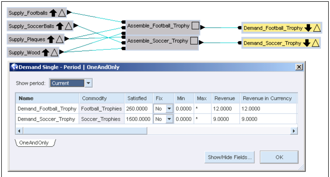
Linear Programming Example, Part 5
