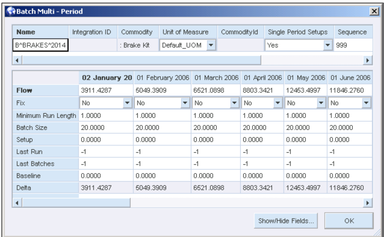
Batch Multi-Period properties window
