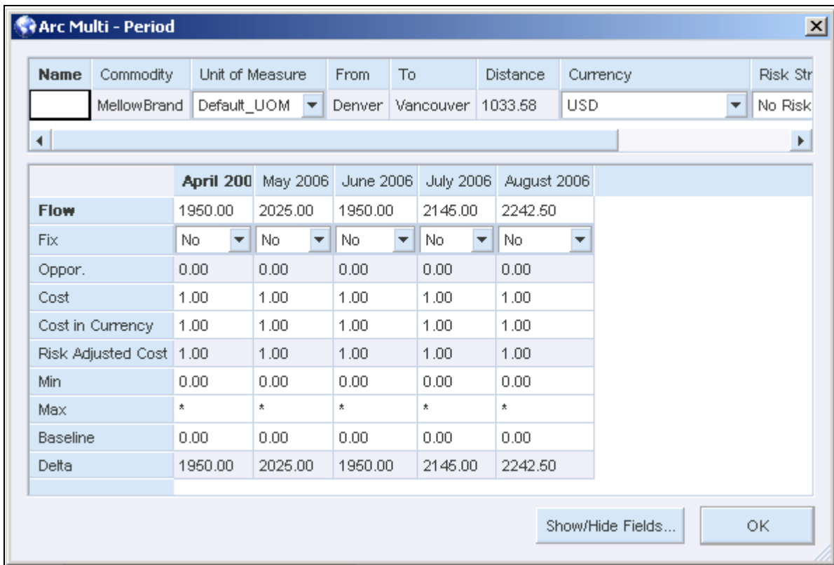
Arc Multi-Period properties window
