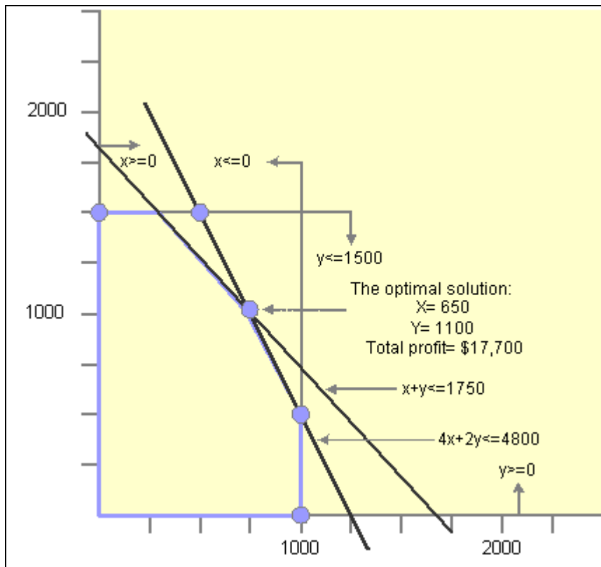
Linear programming example
