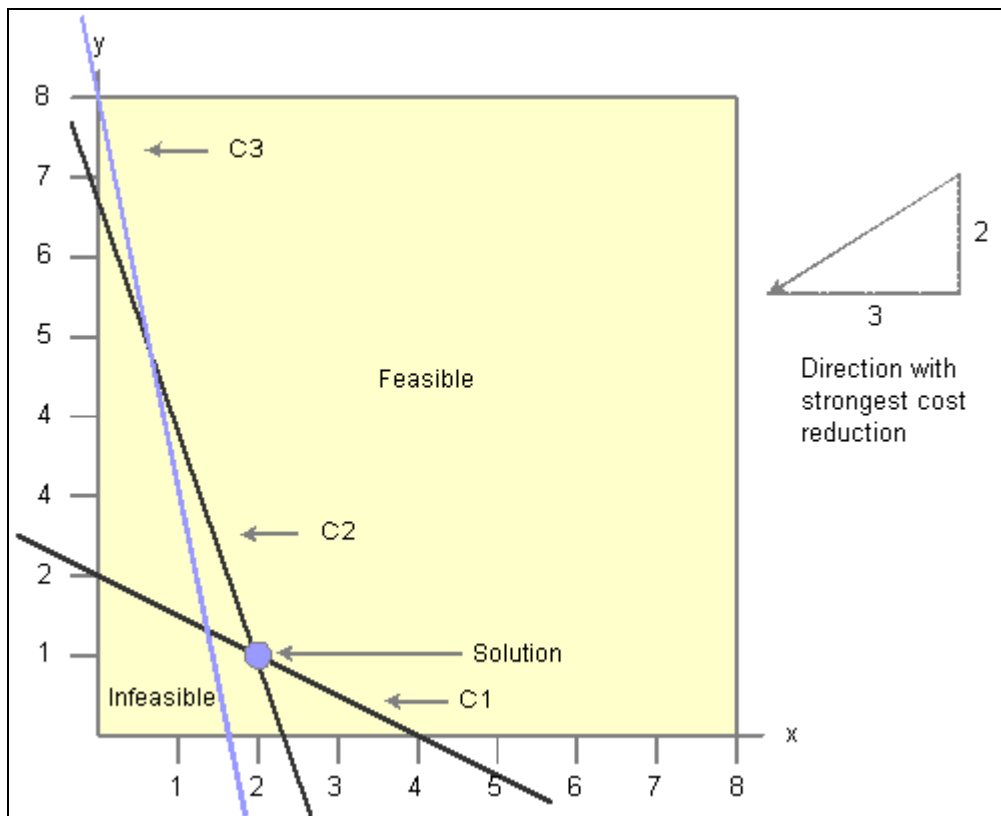
Linear programming example
