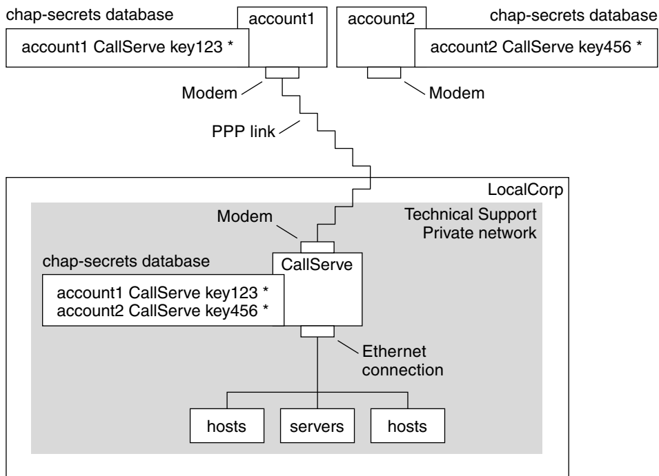
FIGURE 16-4 Example of a CHAP Authentication Scenario (Calling a Private Network)
