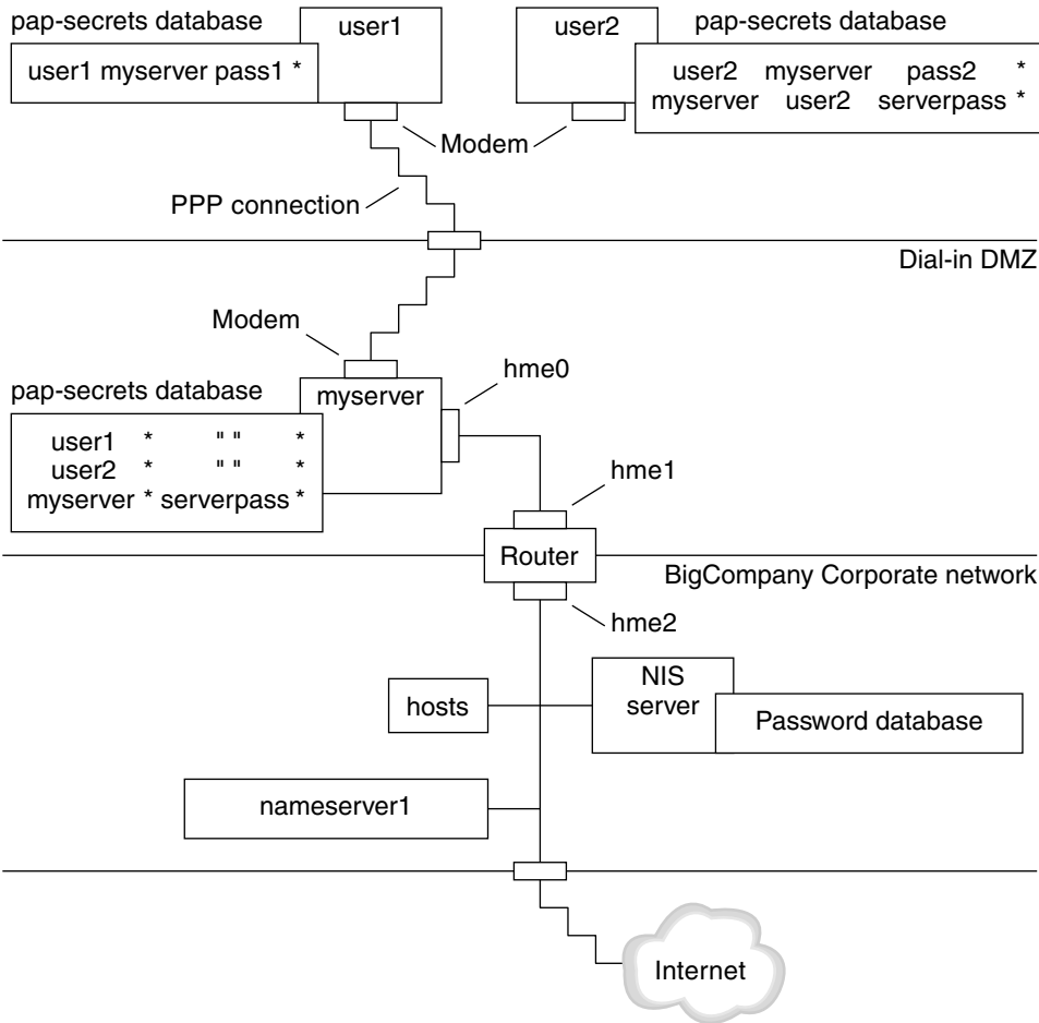
FIGURE 16-3 Example of a PAP Authentication Scenario (Working From Home)
