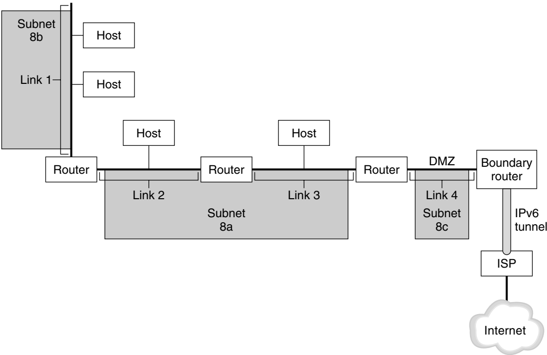
FIGURE 3-1 Basic Components of an IPv6 Network
