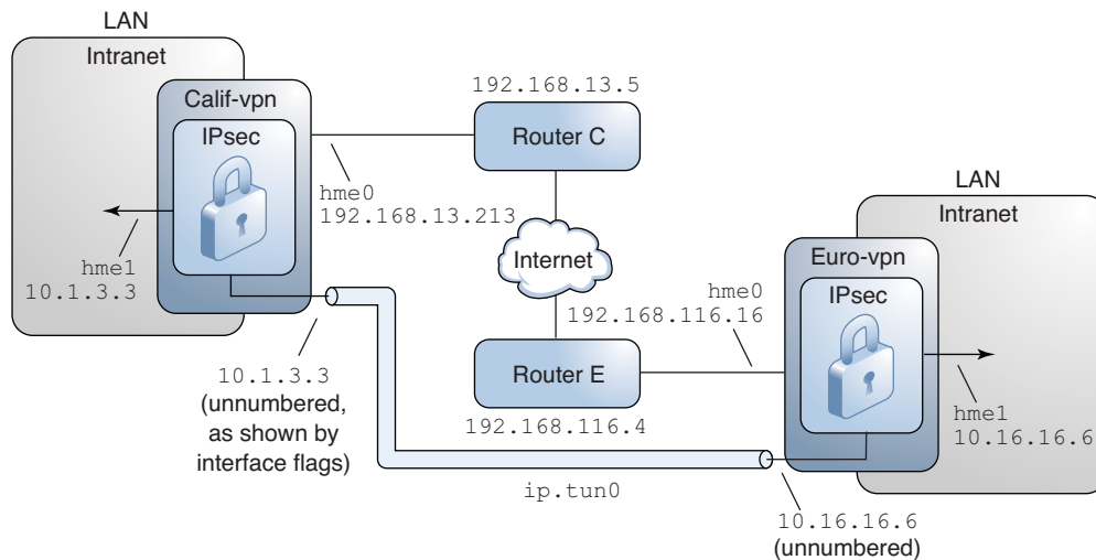
FIGURE 20–2 Sample VPN Between Offices Separated by the Internet
